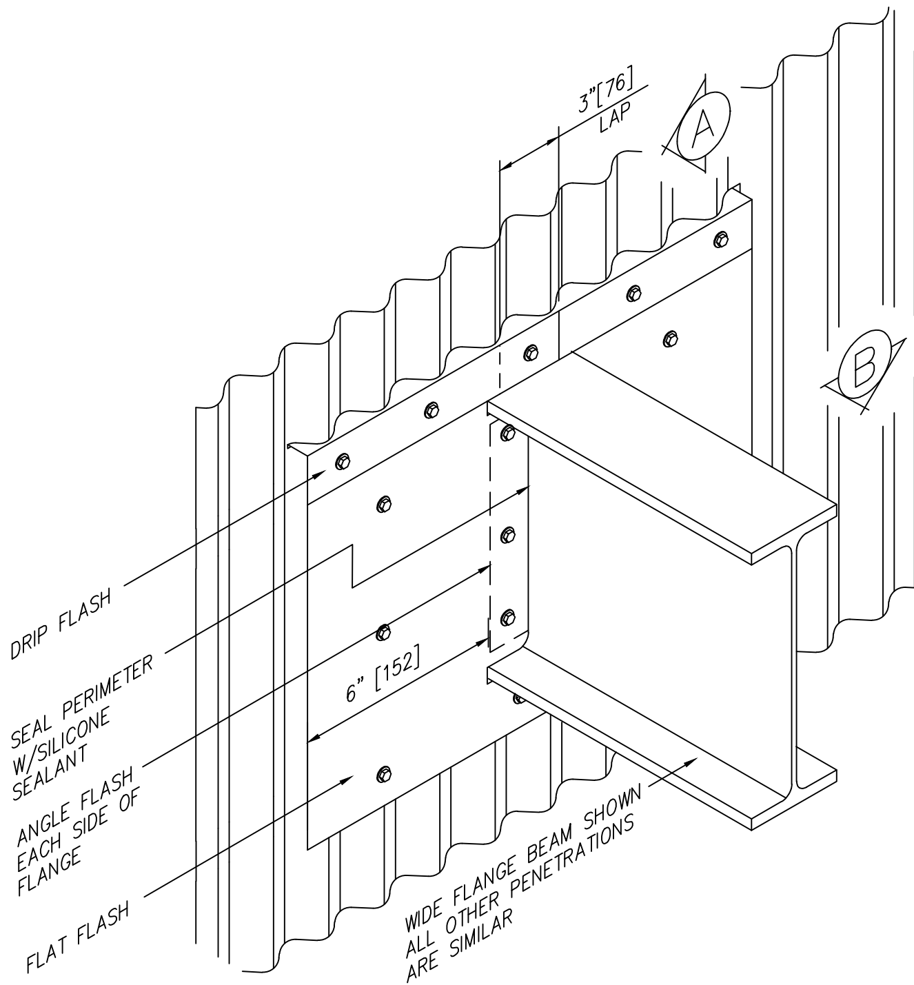
DETAIL 15 PENETRATION
