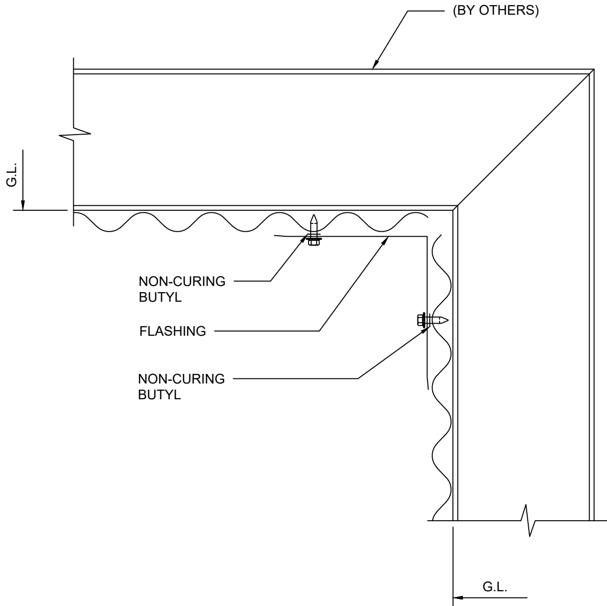
DETAIL 10 INSIDE CORNER
