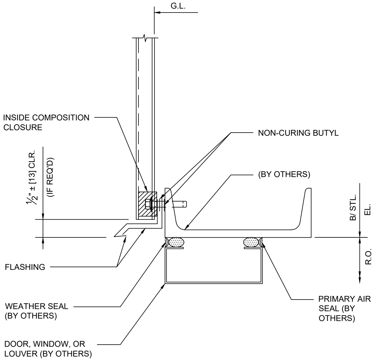
DETAIL 4 HEAD OPENING
