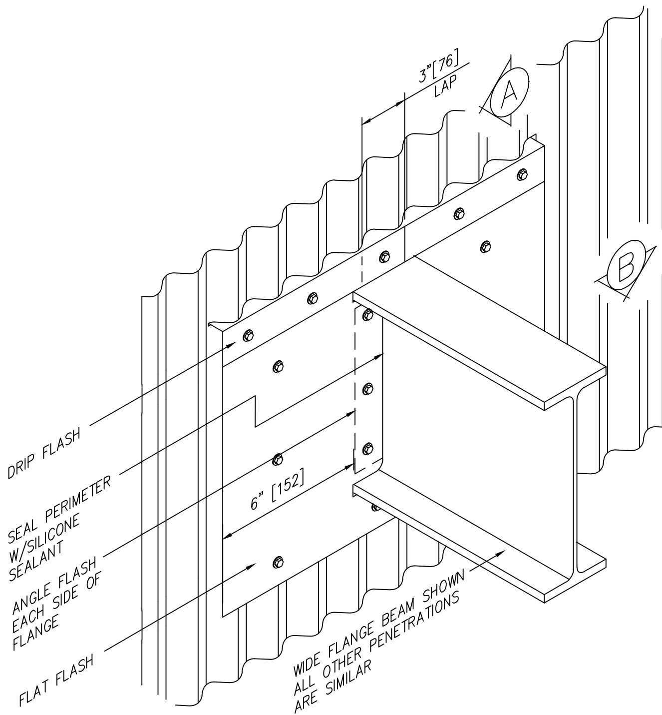
DETAIL 15 PENETRATION
