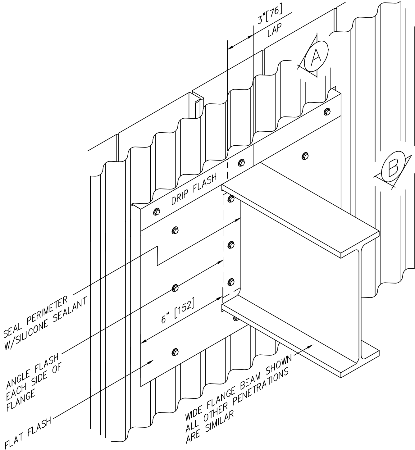
DETAIL 15C PENETRATION
