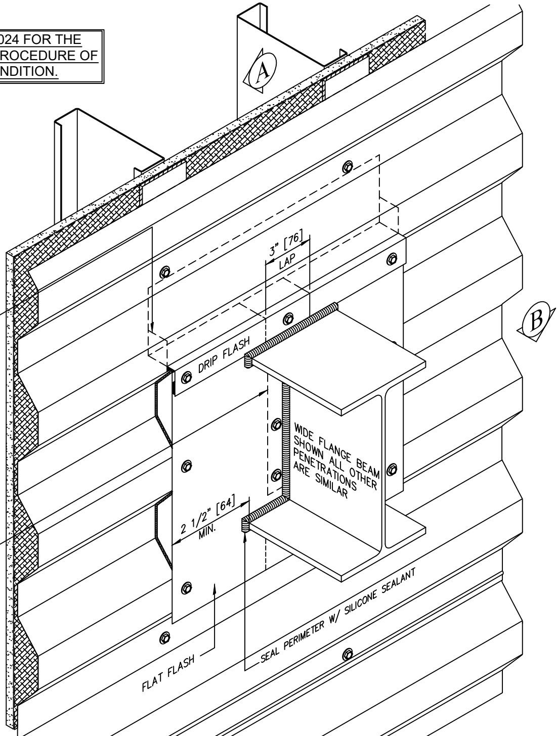
DETAIL 15 PENETRATION
