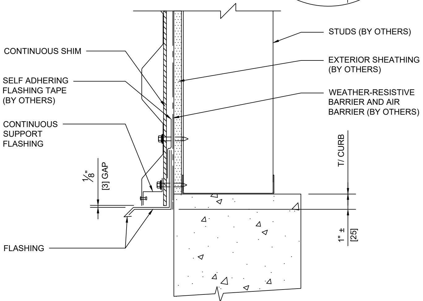
DETAIL 3B BASE @ CURB (HIGH CELL)
