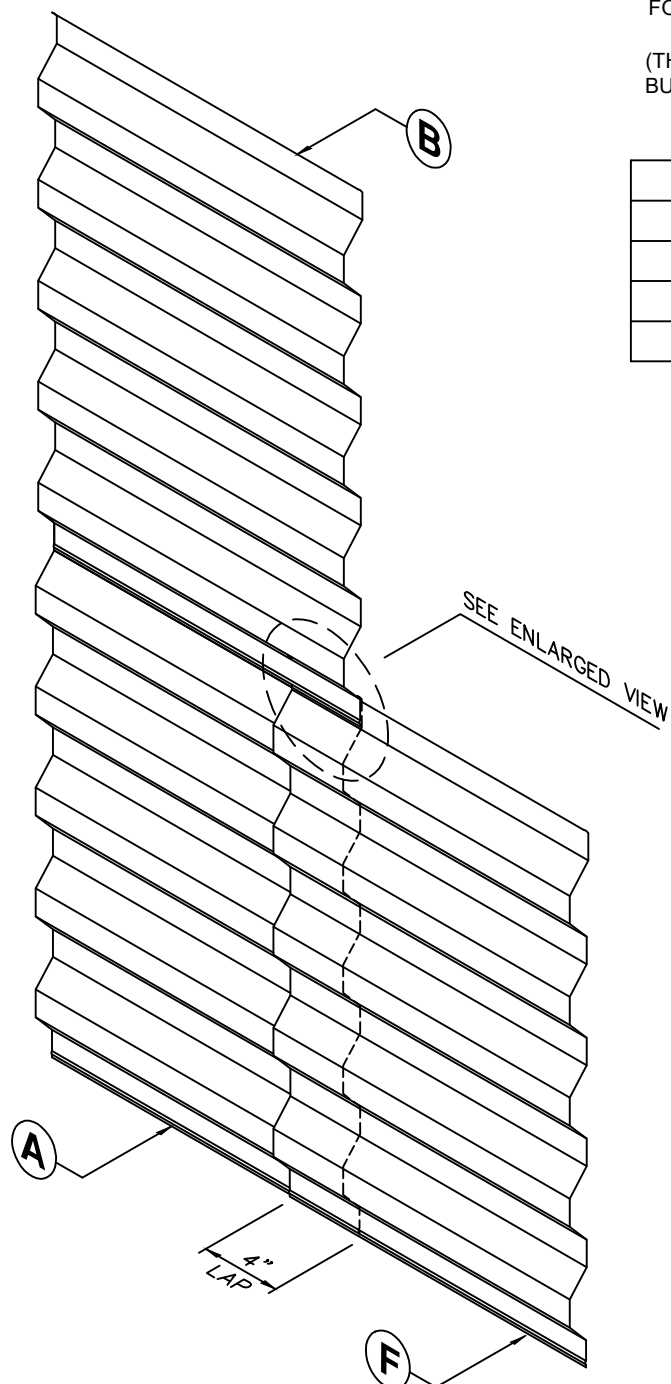
DETAIL 2C ERECTION SEQUENCE
