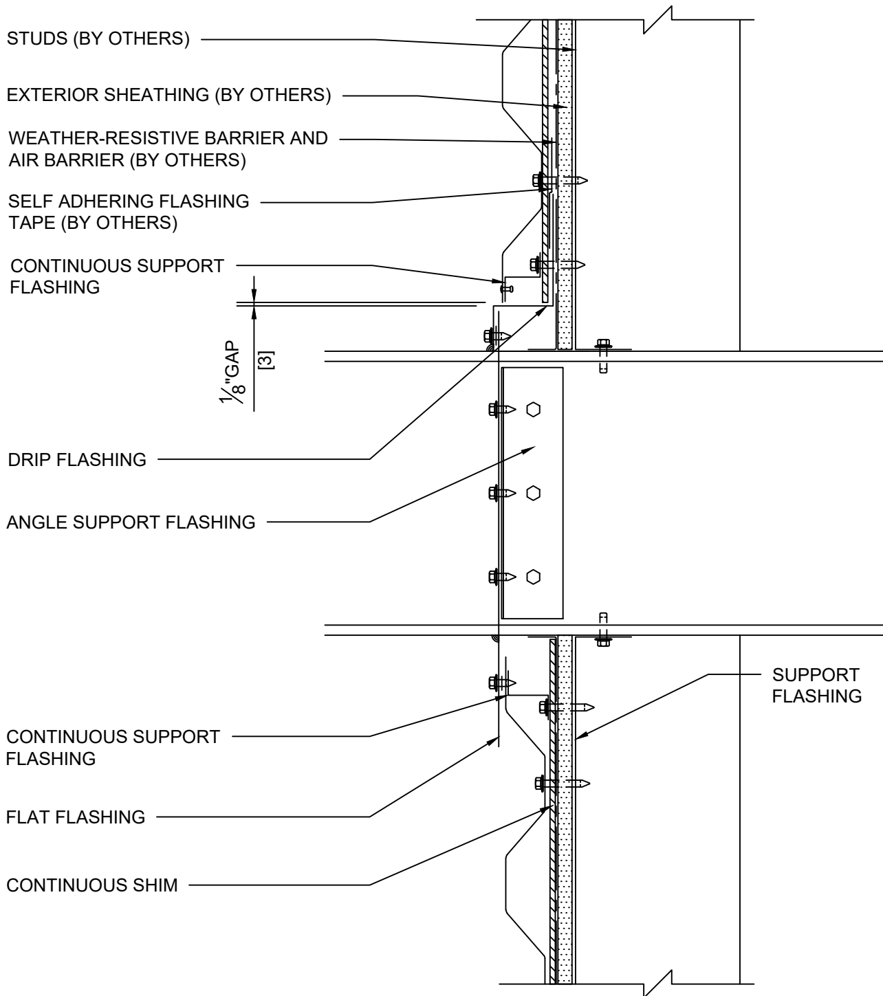
DETAIL 15A PENETRATION (SECTION A-A)
