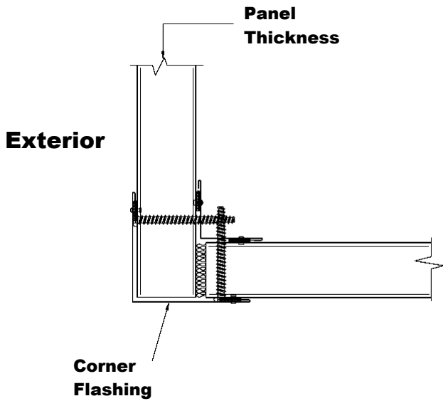
Corner-Flashing
