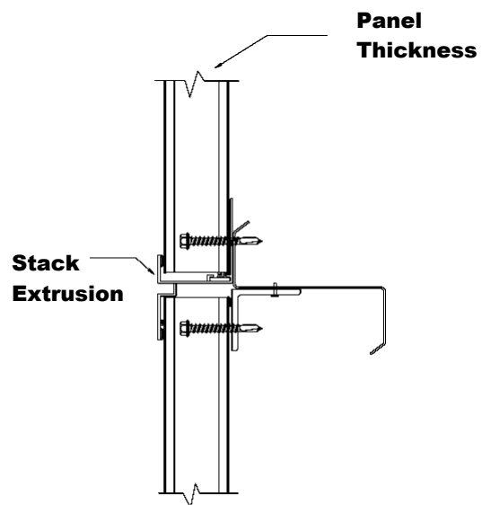
Stack-Extrusion
