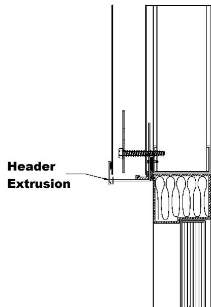
Header Extrusion
