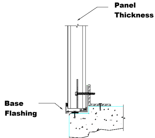
Base-Extrusion
