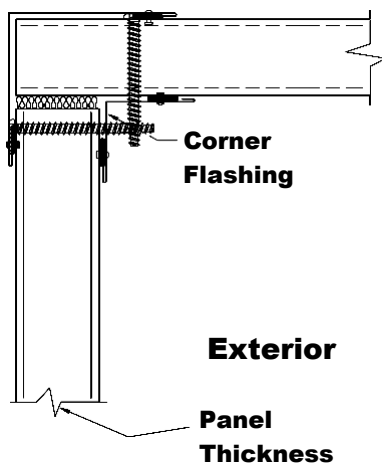
90° Inside Corner-Flashing
