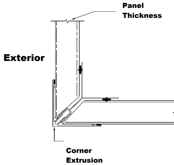
Corner-Extrusion
