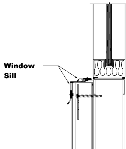
Window Sill
