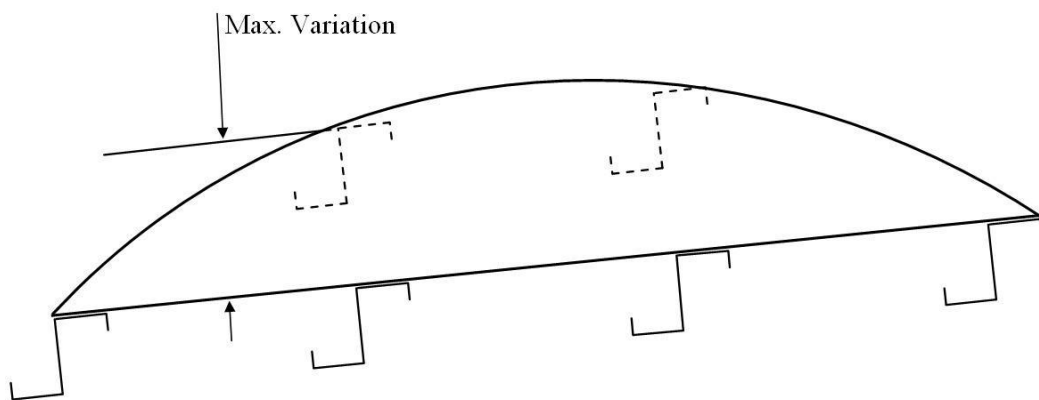
Mis-Alignment (Avoid these Conditions)
