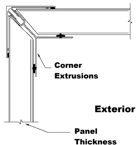
90° Inside Corner-Extrusion
