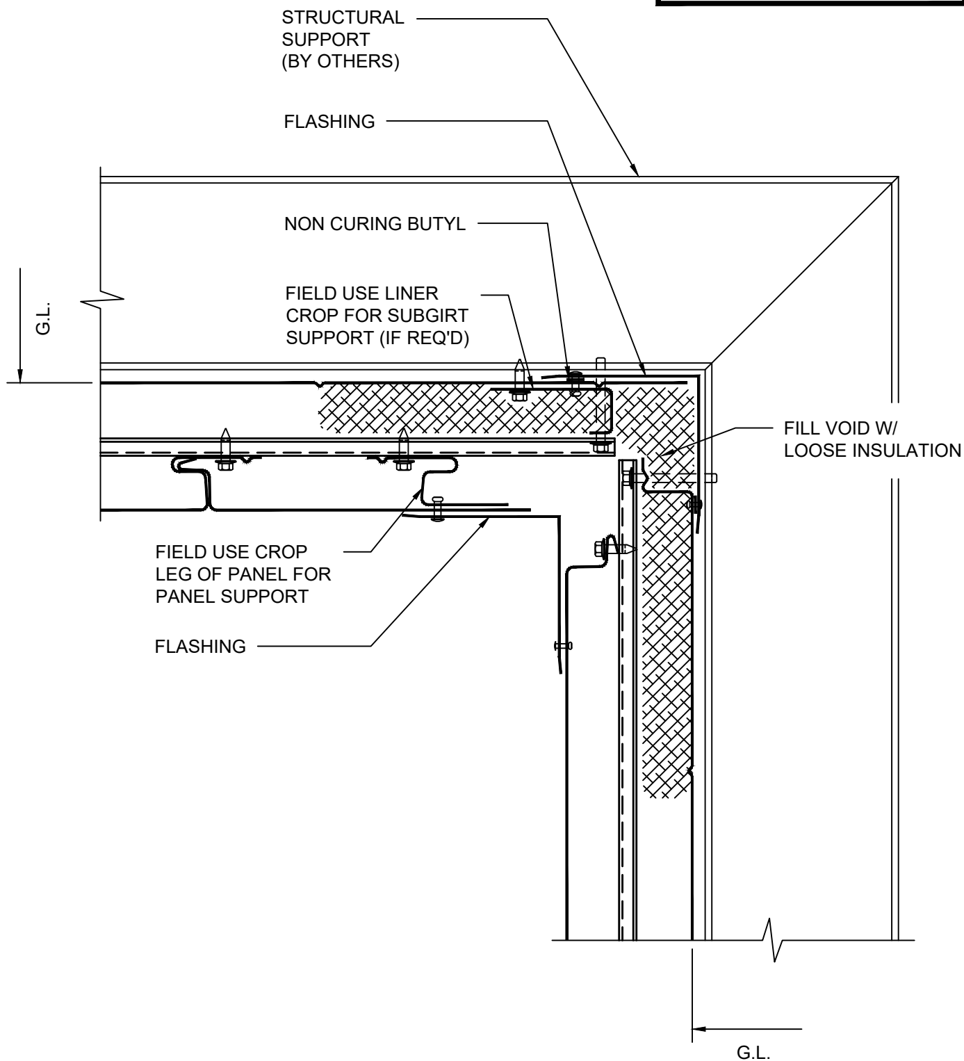
DETAIL 10 I.S. CORNER
