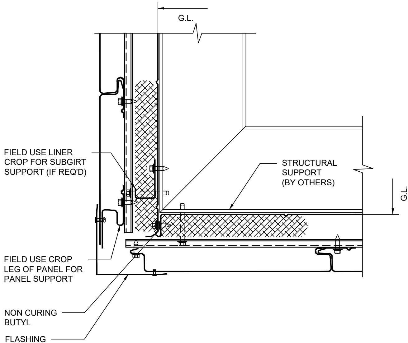
DETAIL 9A O.S. CORNER (ALTERNATE)
