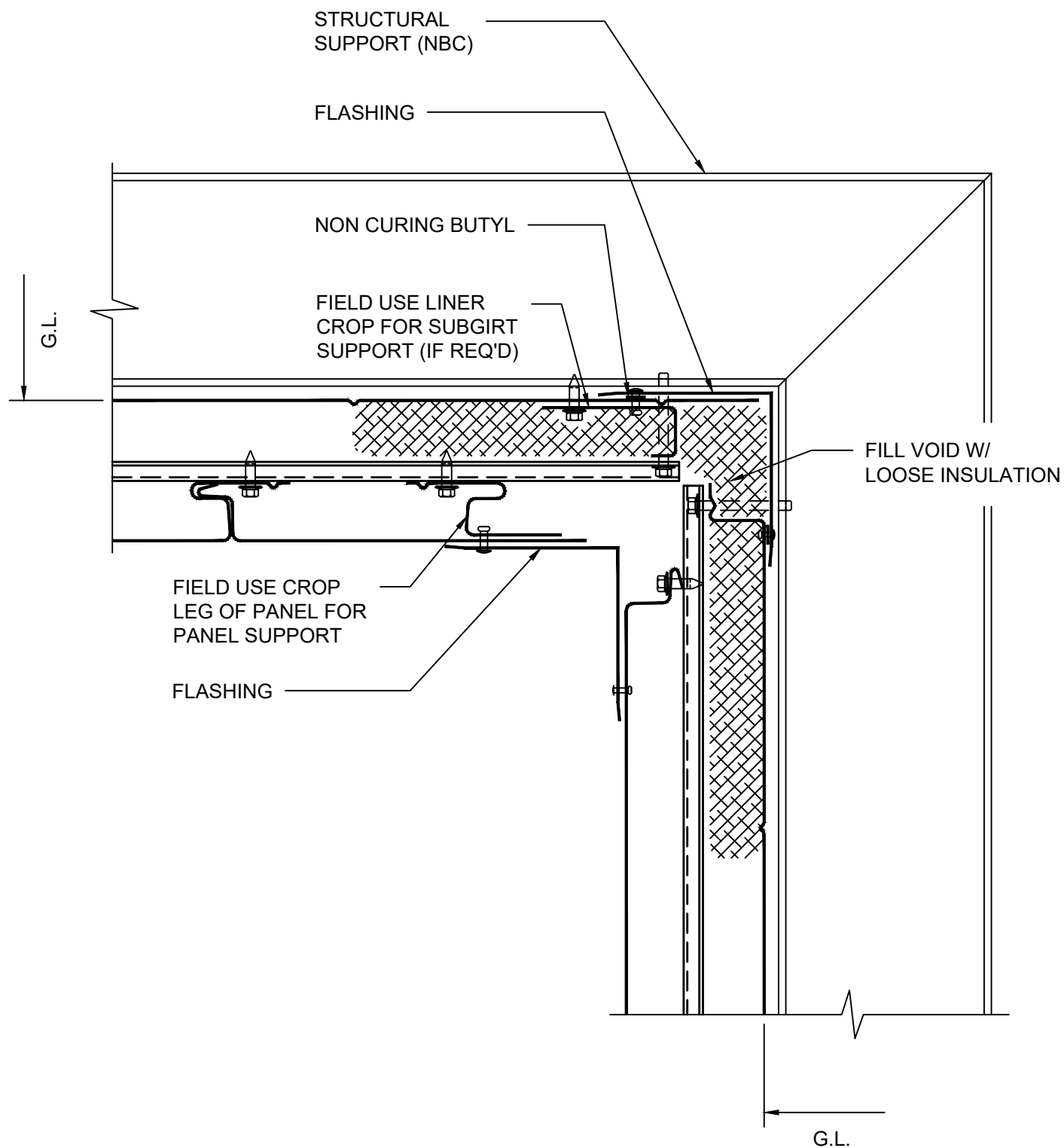
DETAIL 10 I.S. CORNER
