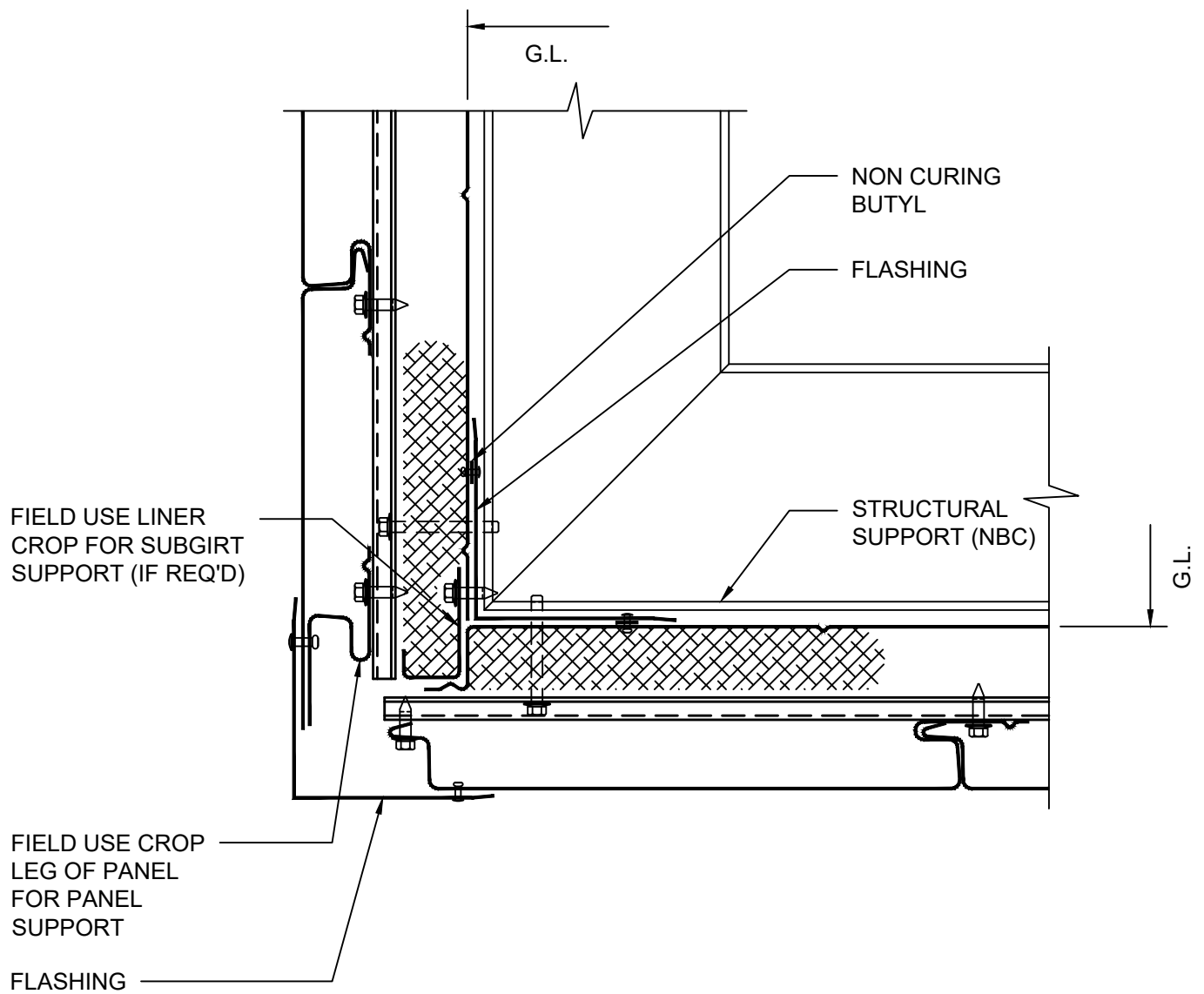
DETAIL 9 O.S. CORNER
