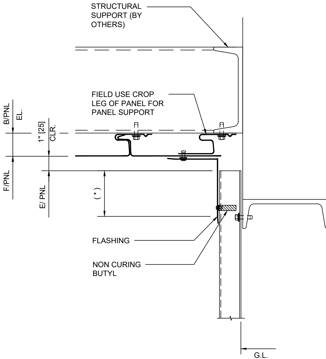
DETAIL 8B SOFFIT / SIDEWALL
