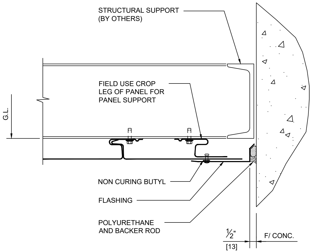
DETAIL 11 ENDWALL
