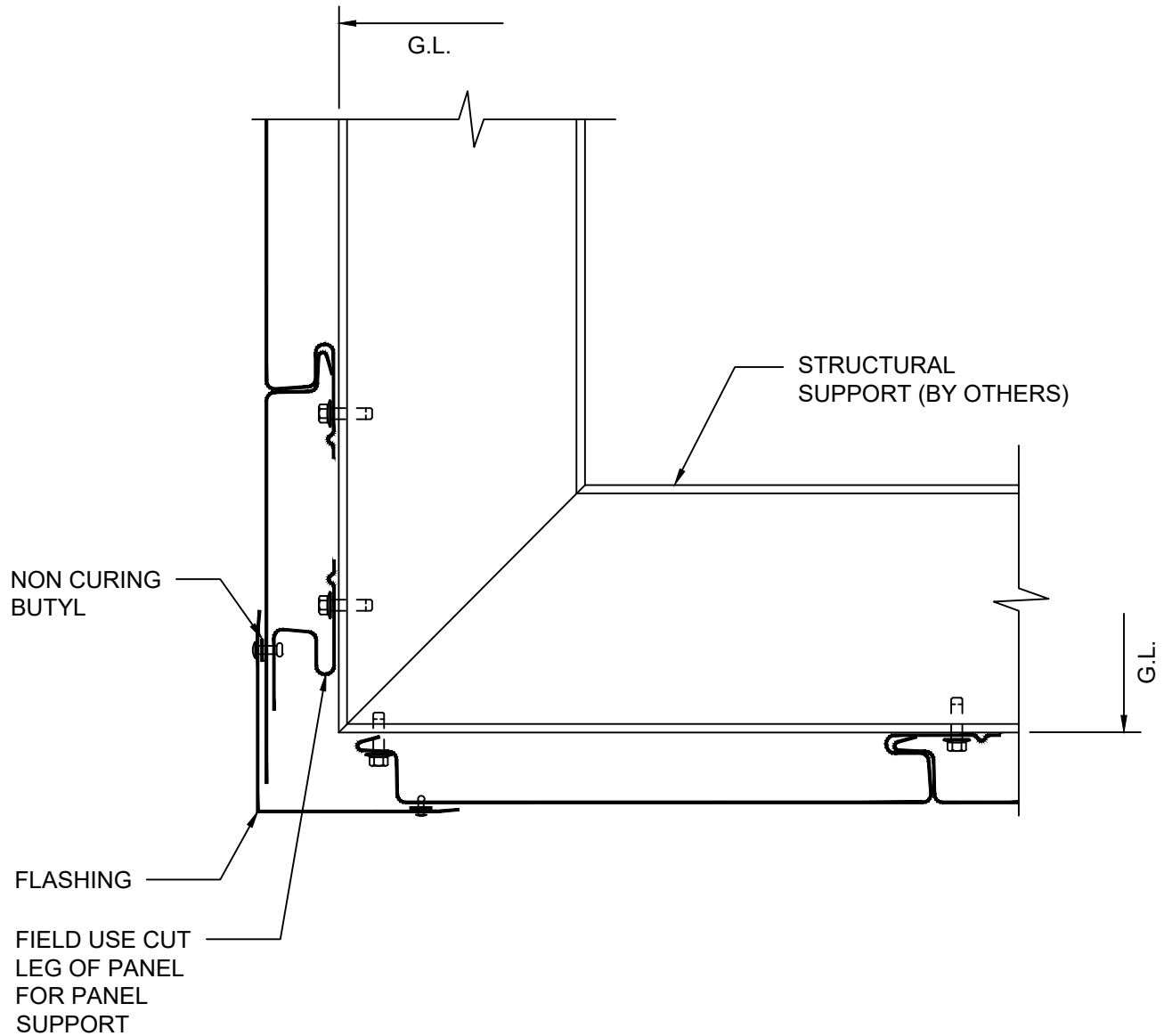
DETAIL 9 O.S. CORNER
