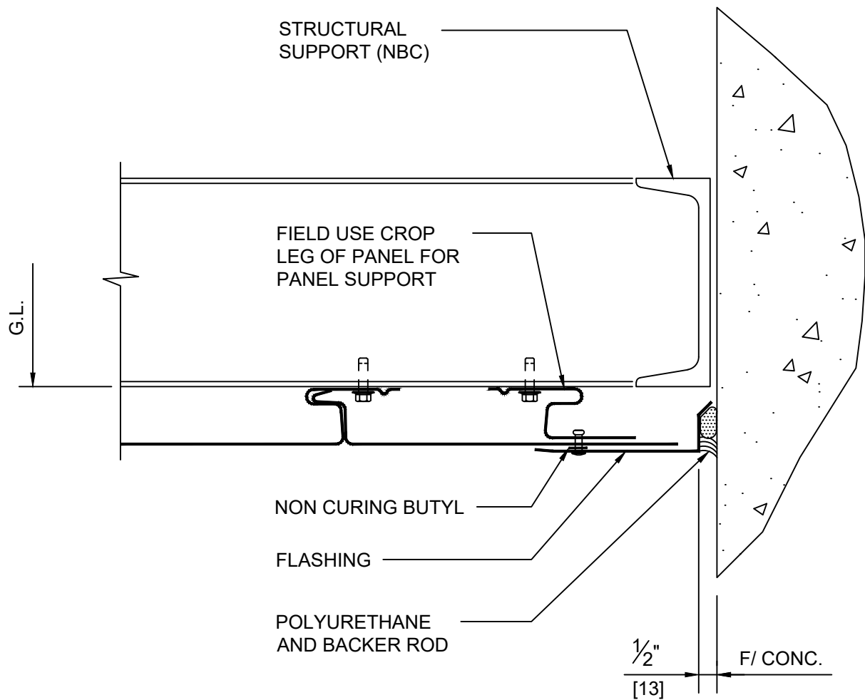
DETAIL 11 ENDWALL
