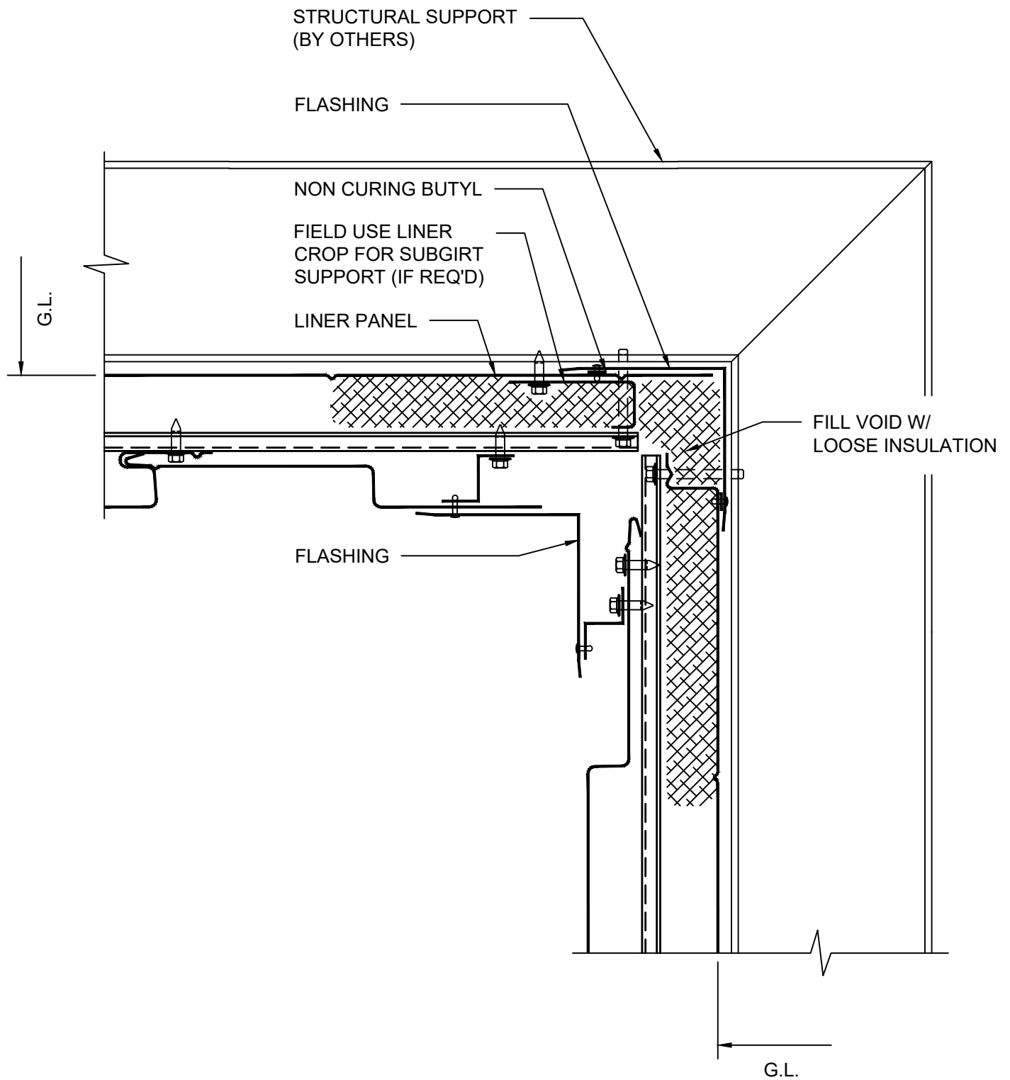
DETAIL 10 I.S. CORNER - INSULATED
