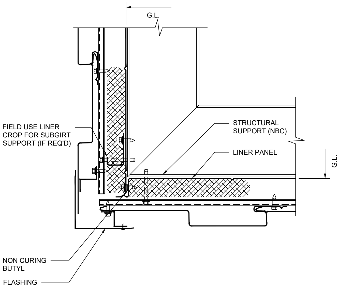
DETAIL 9A O.S. CORNER - WITHOUT LINER FLASH - INSULATED
