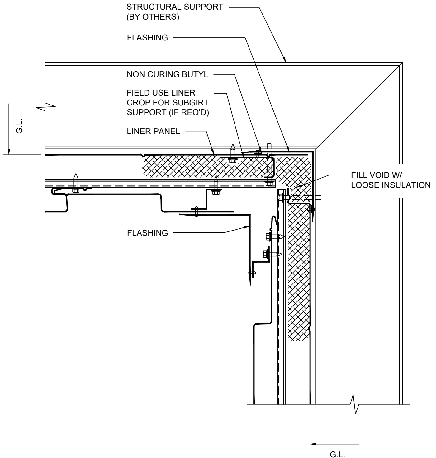
DETAIL 10 I.S. CORNER - INSULATED
