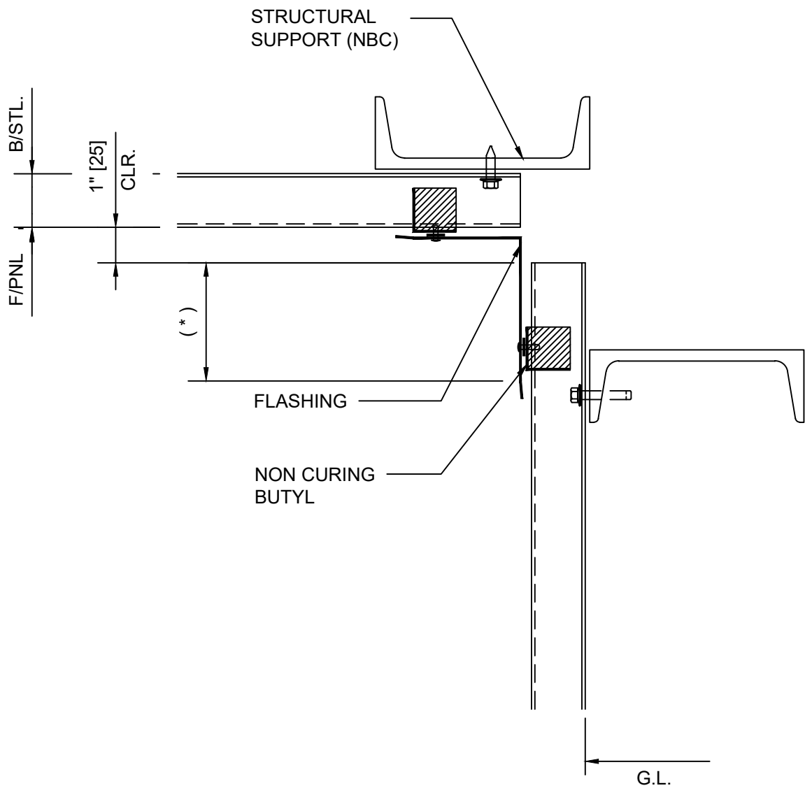
DETAIL 8A SOFFIT/ BACKWALL
