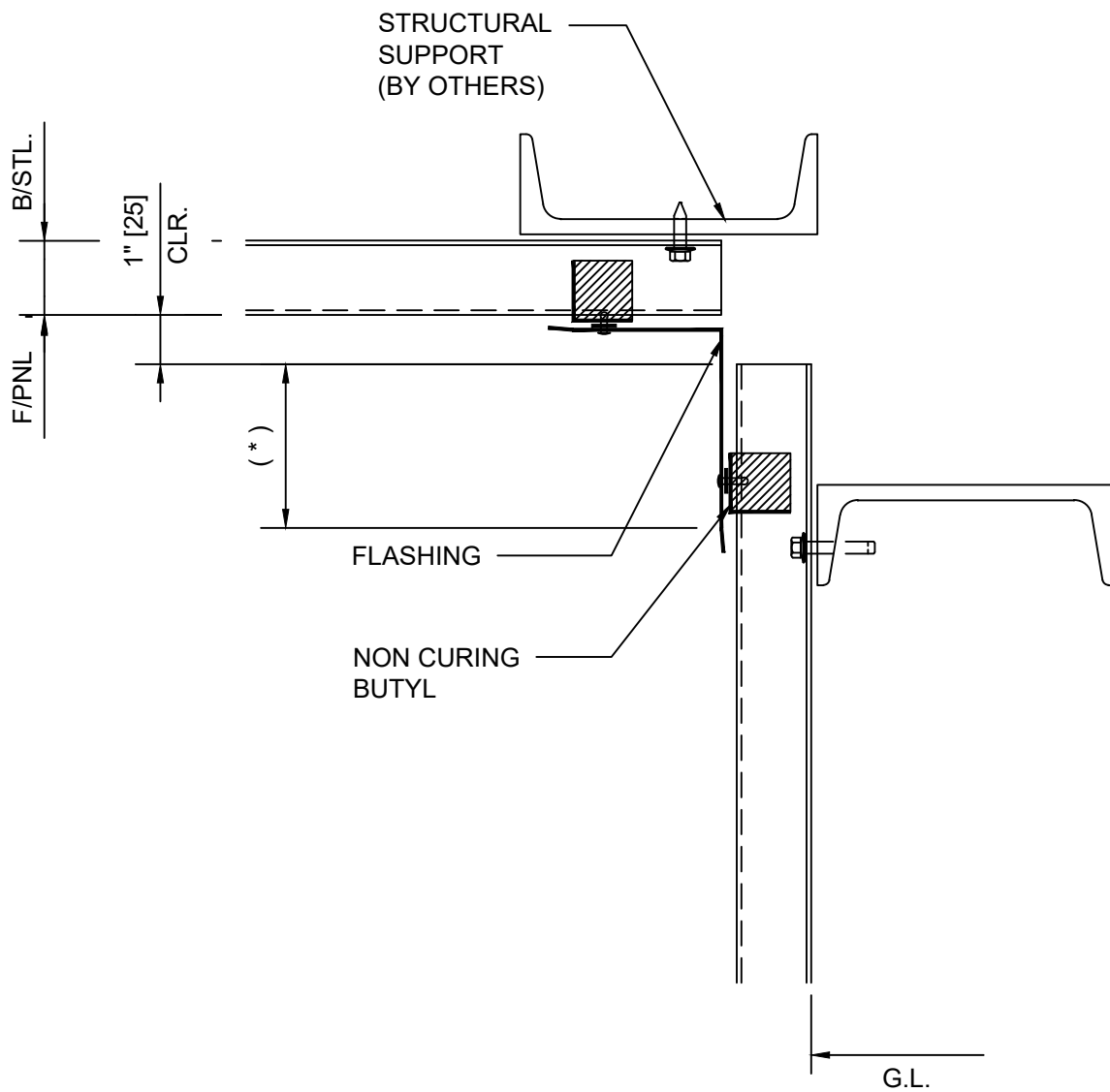
DETAIL 8A SOFFIT/ BACKWALL
