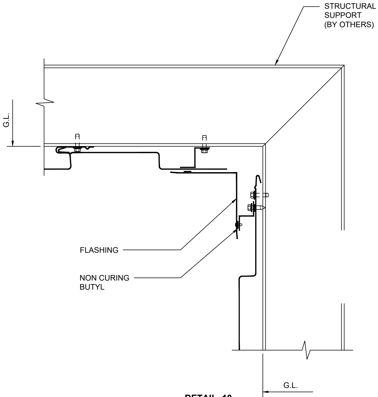
DETAIL 10 I.S. CORNER
