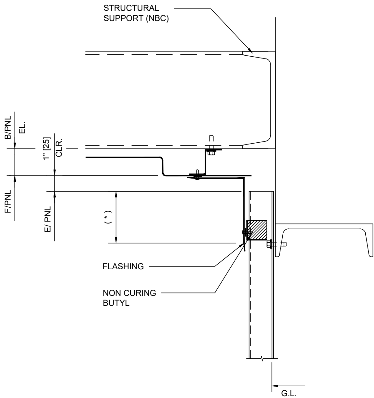
DETAIL 8B SOFFIT / SIDEWALL
