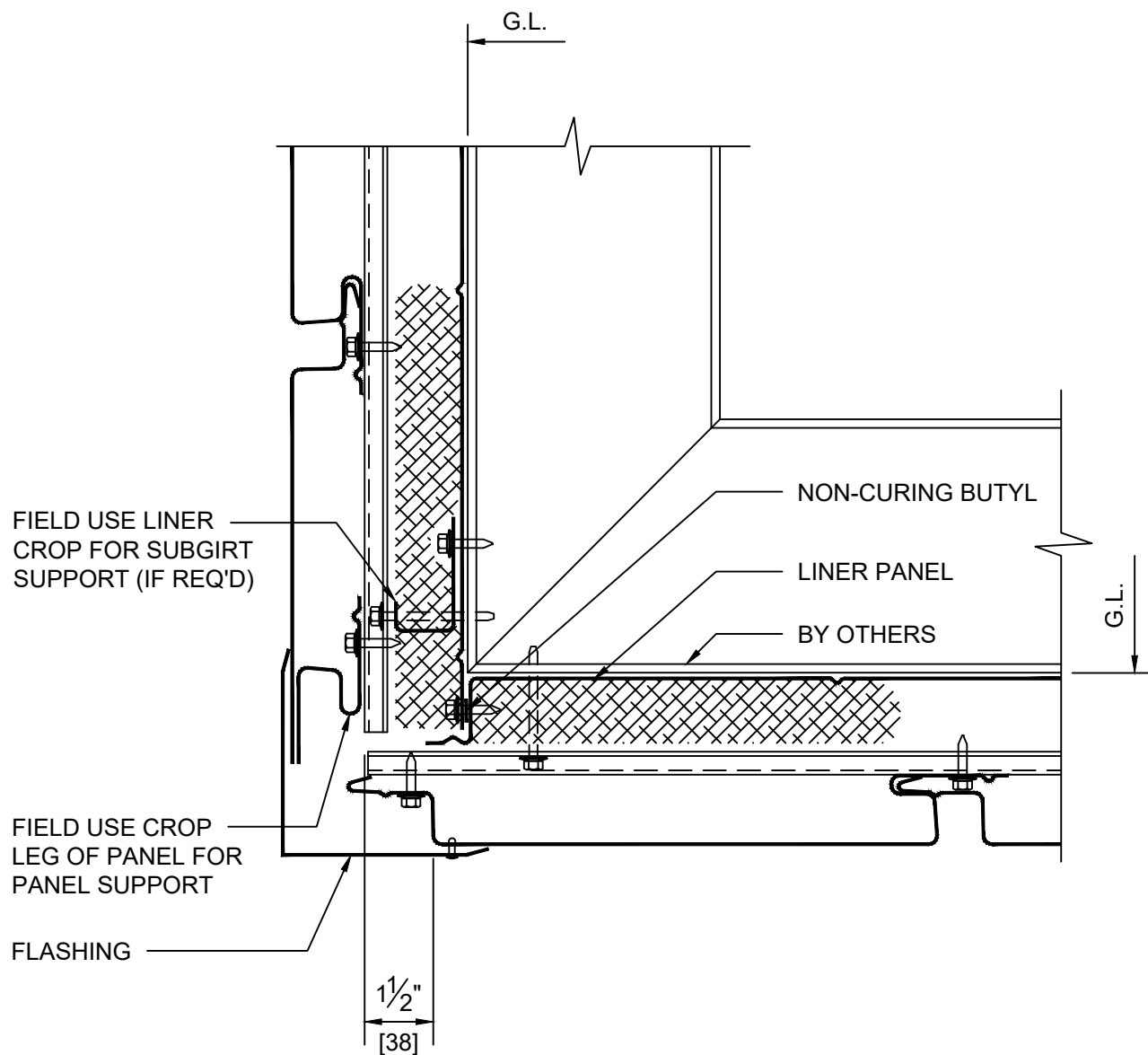
DETAIL 9A OUTSIDE CORNER - WITHOUT LINER FLASH - INSULATED
