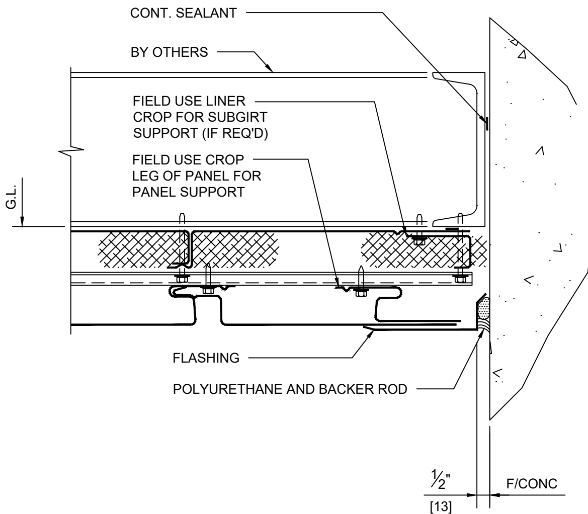
DETAIL 11 ENDWALL
