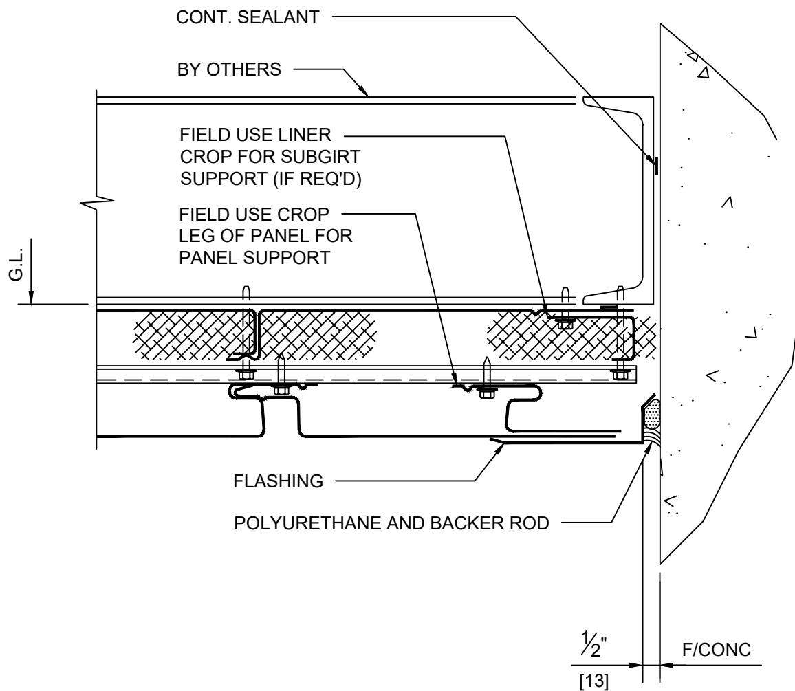
DETAIL 11 ENDWALL
