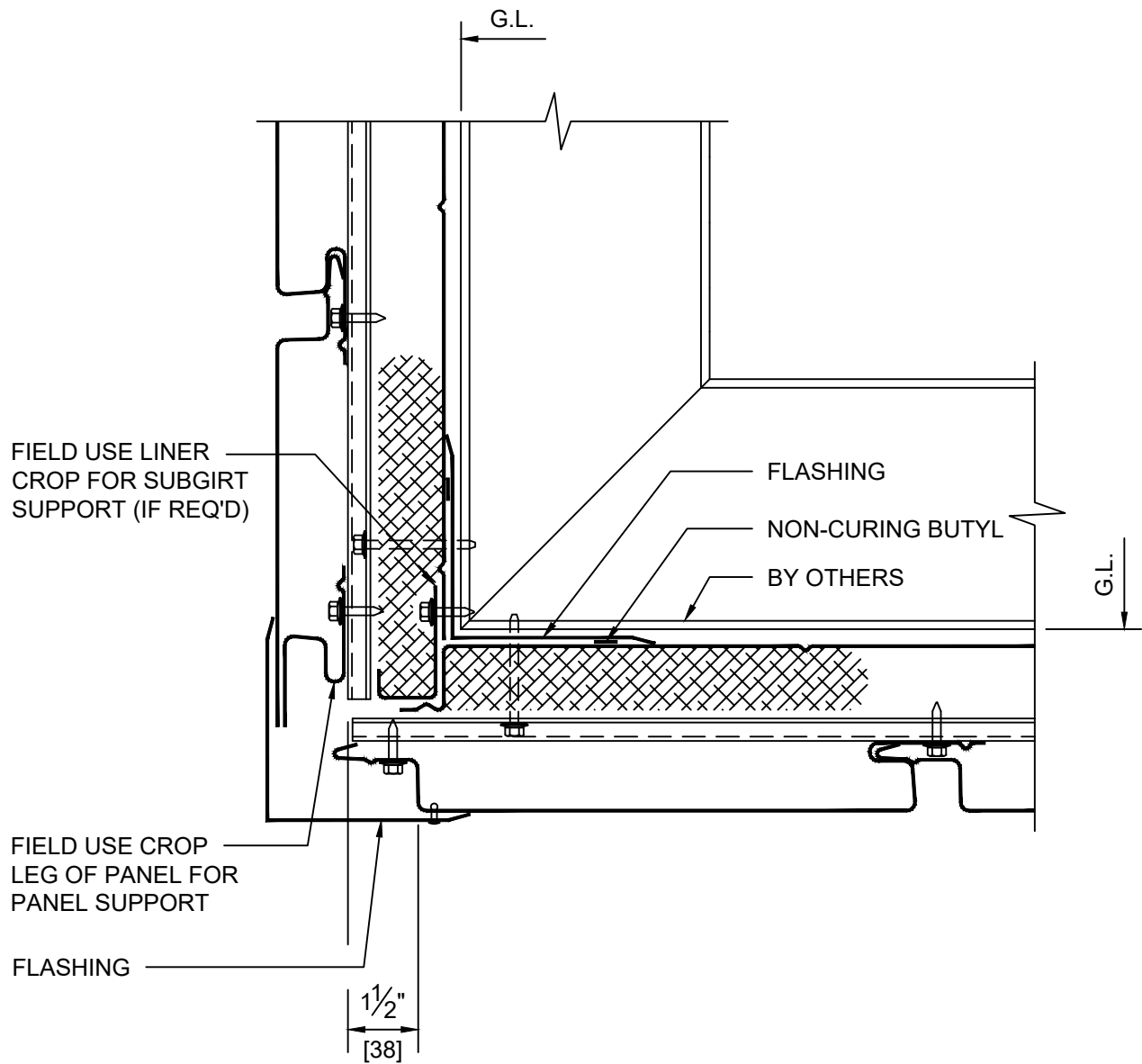
DETAIL 9 OUTSIDE CORNER - WITH LINER FLASH - INSULATED
