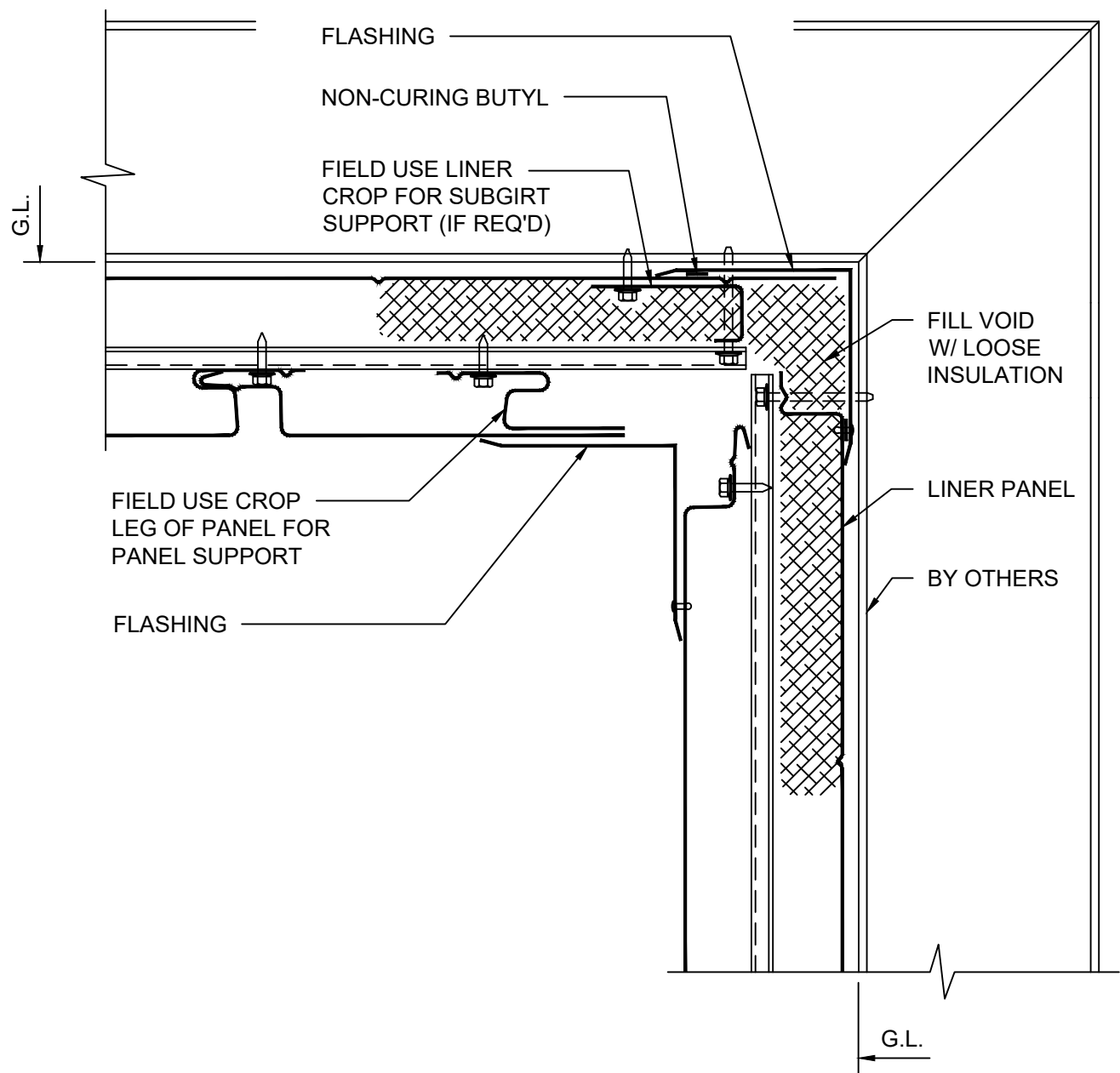
DETAIL 10 INSIDE CORNER - INSULATED
