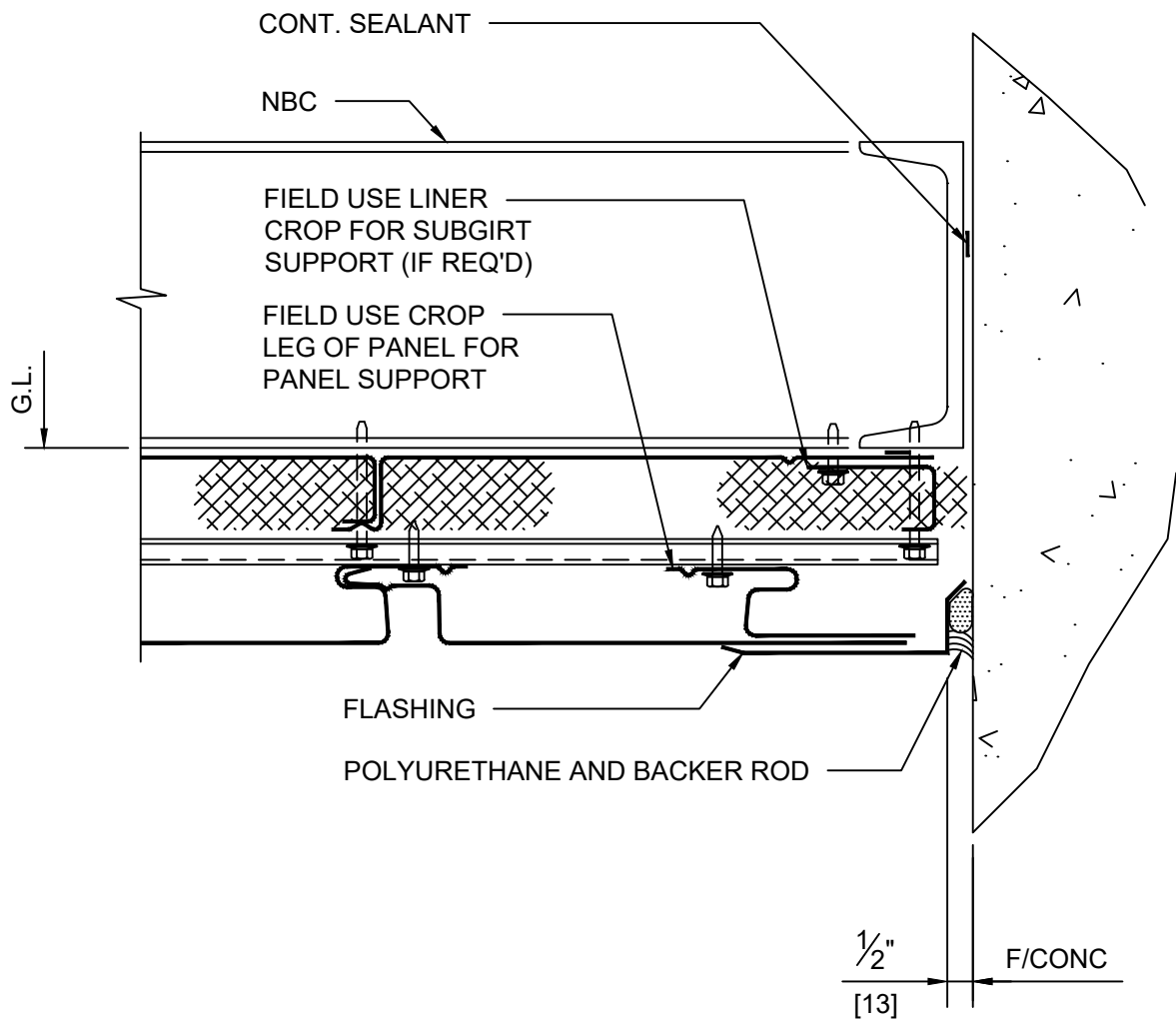
DETAIL 11 ENDWALL
