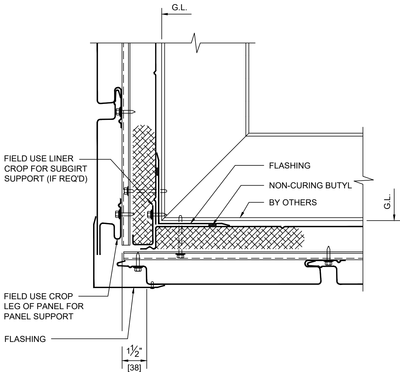
DETAIL 9 OUTSIDE CORNER - WITH LINER FLASH - INSULATED
