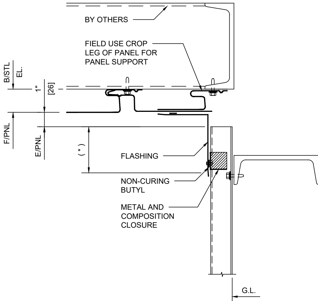
DETAIL 8B SOFFIT/SIDEWALL
