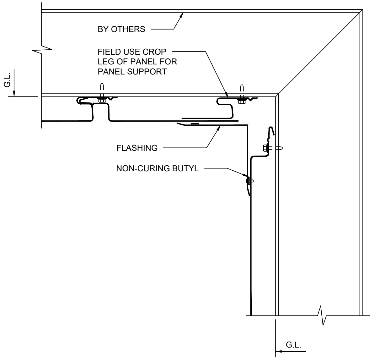
DETAIL 10 INSIDE CORNER
