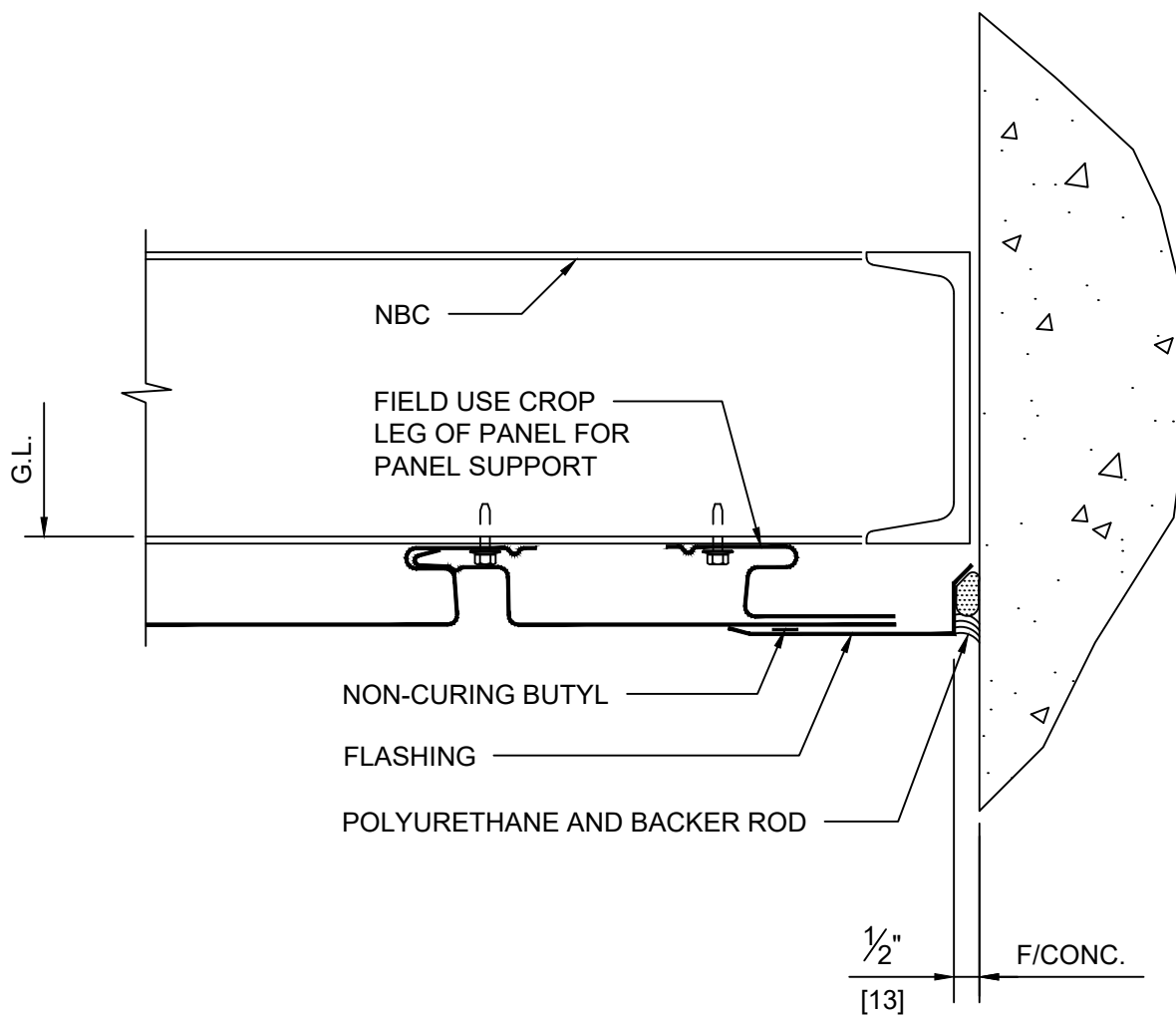
DETAIL 11 ENDWALL
