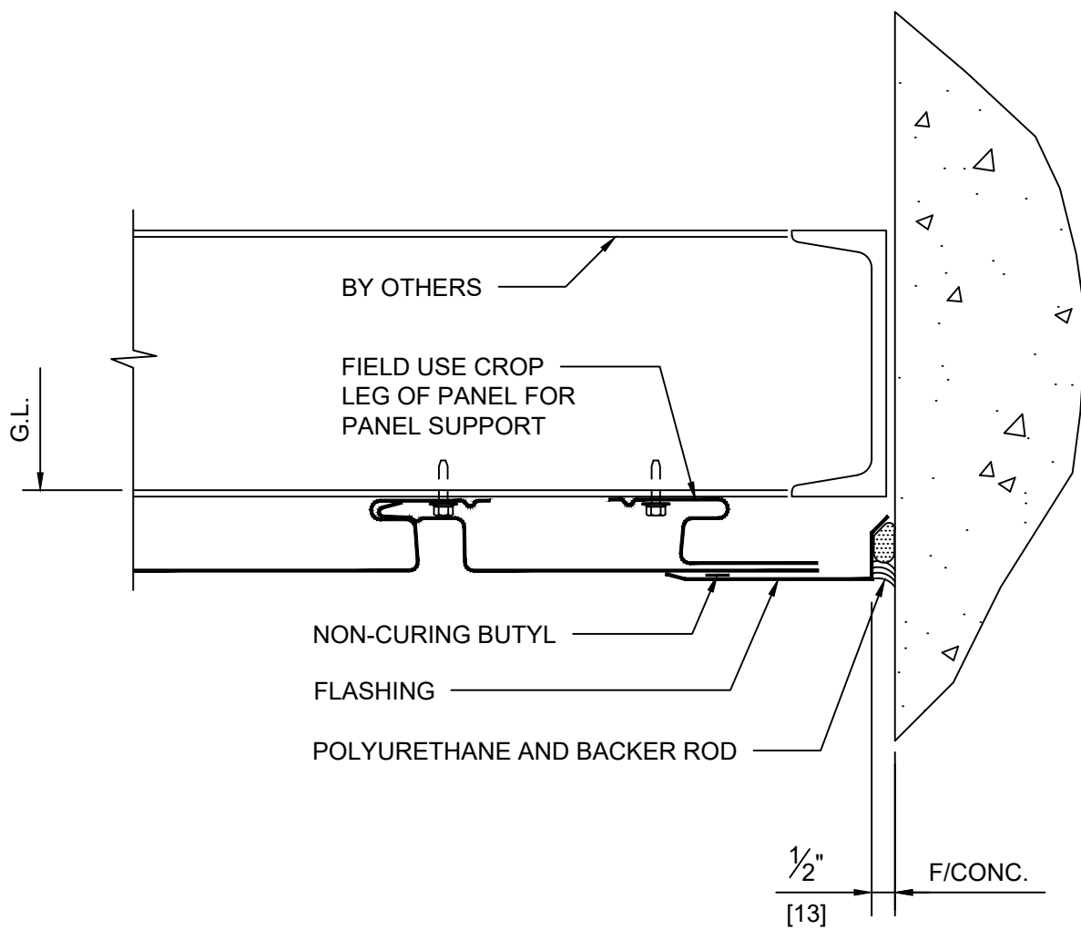
DETAIL 11 ENDWALL
