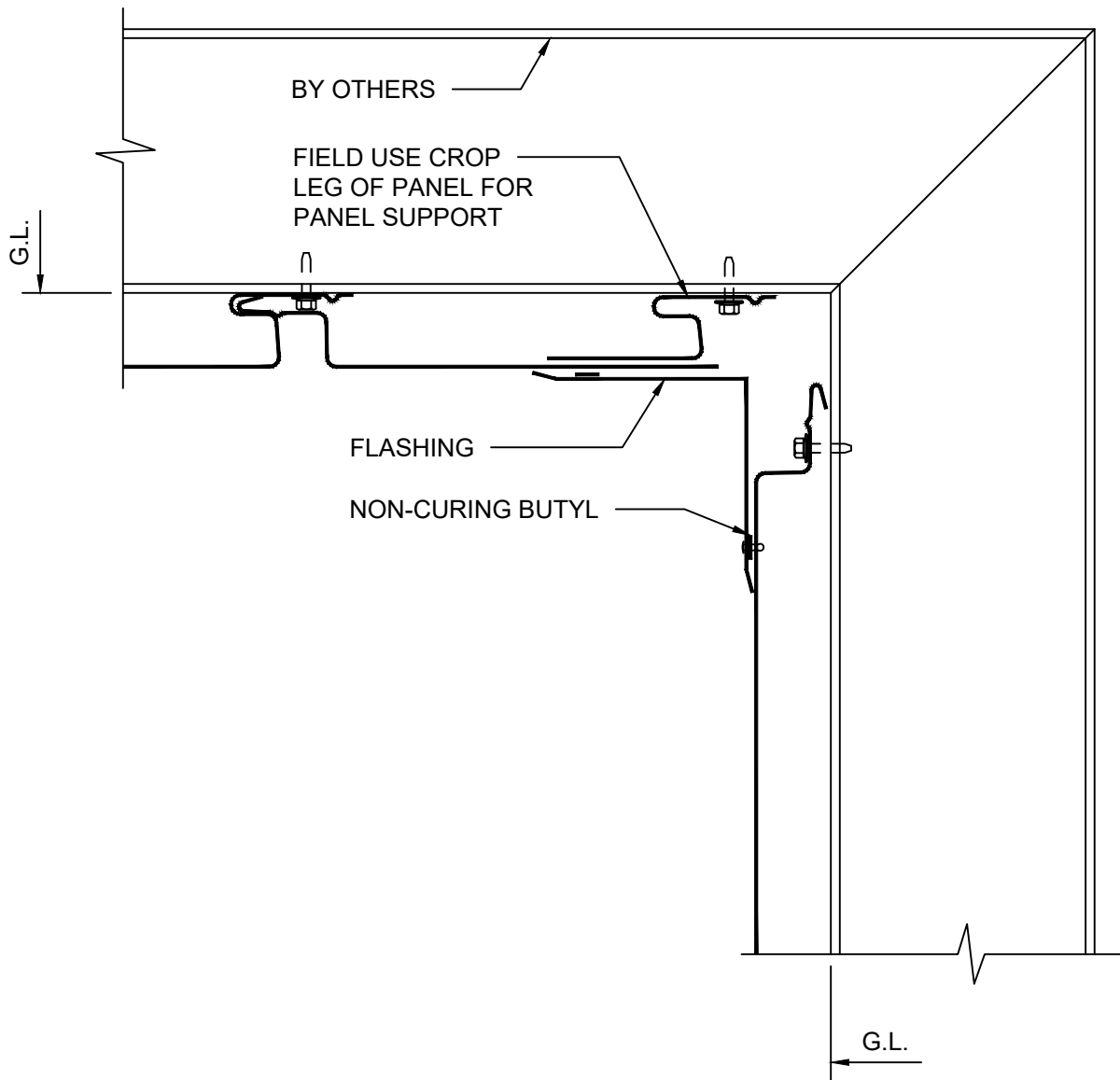
DETAIL 10 INSIDE CORNER
