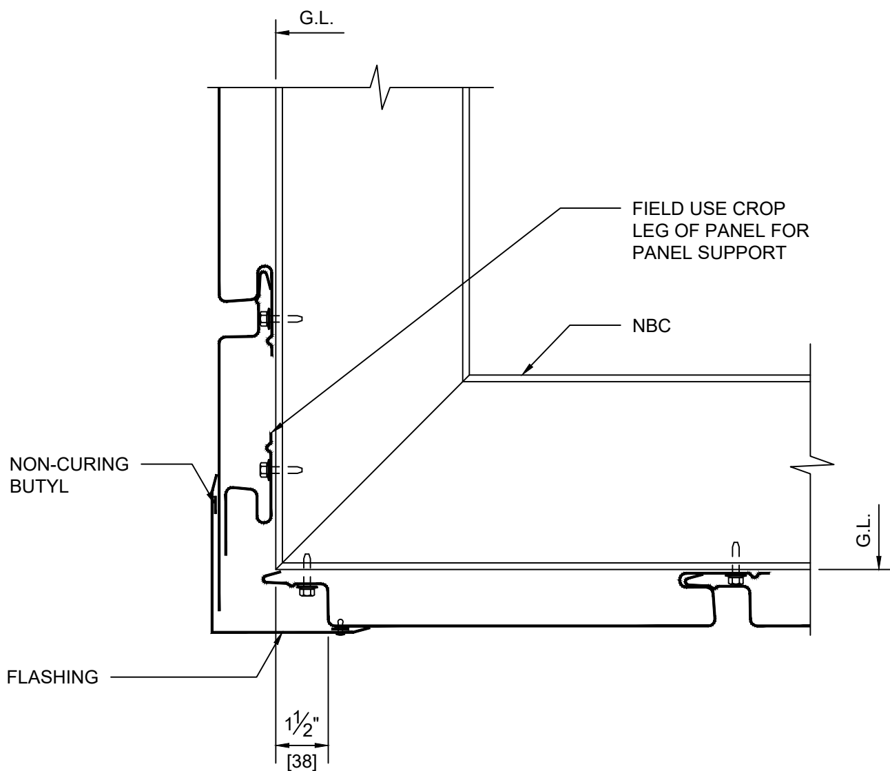
DETAIL 9 OUTSIDE CORNER
