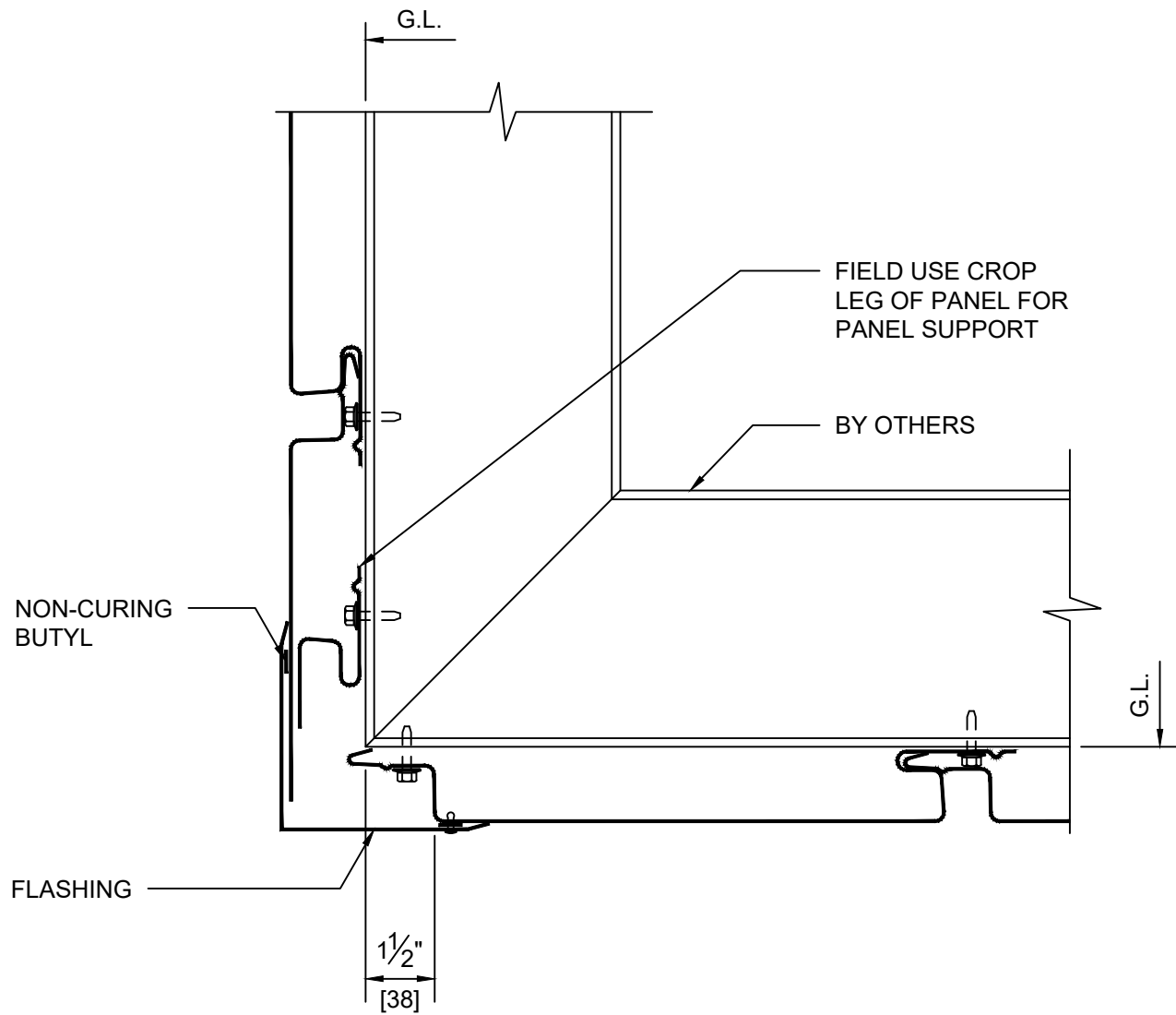
DETAIL 9 OUTSIDE CORNER
