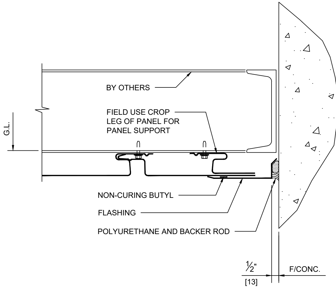
DETAIL 11 ENDWALL
