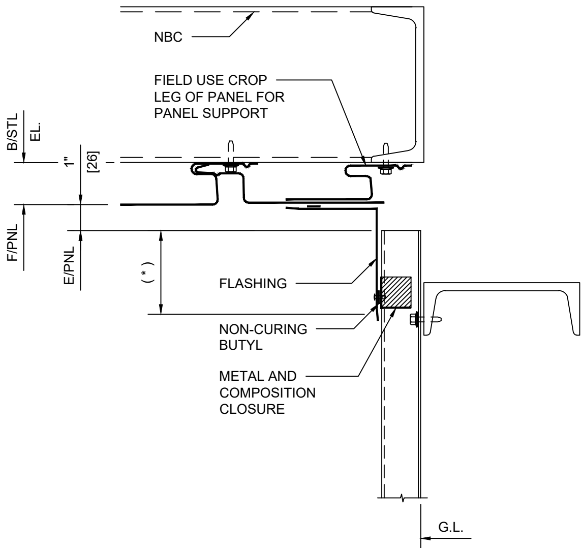
DETAIL 8B SOFFIT/SIDEWALL
