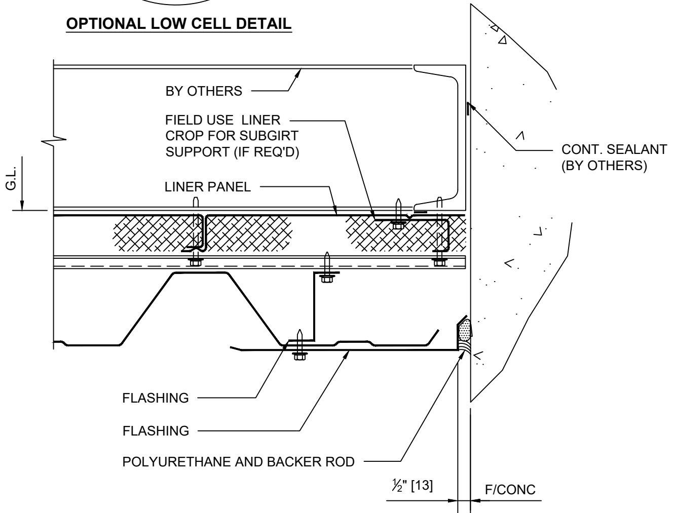
DETAIL 11 ENDWALL
