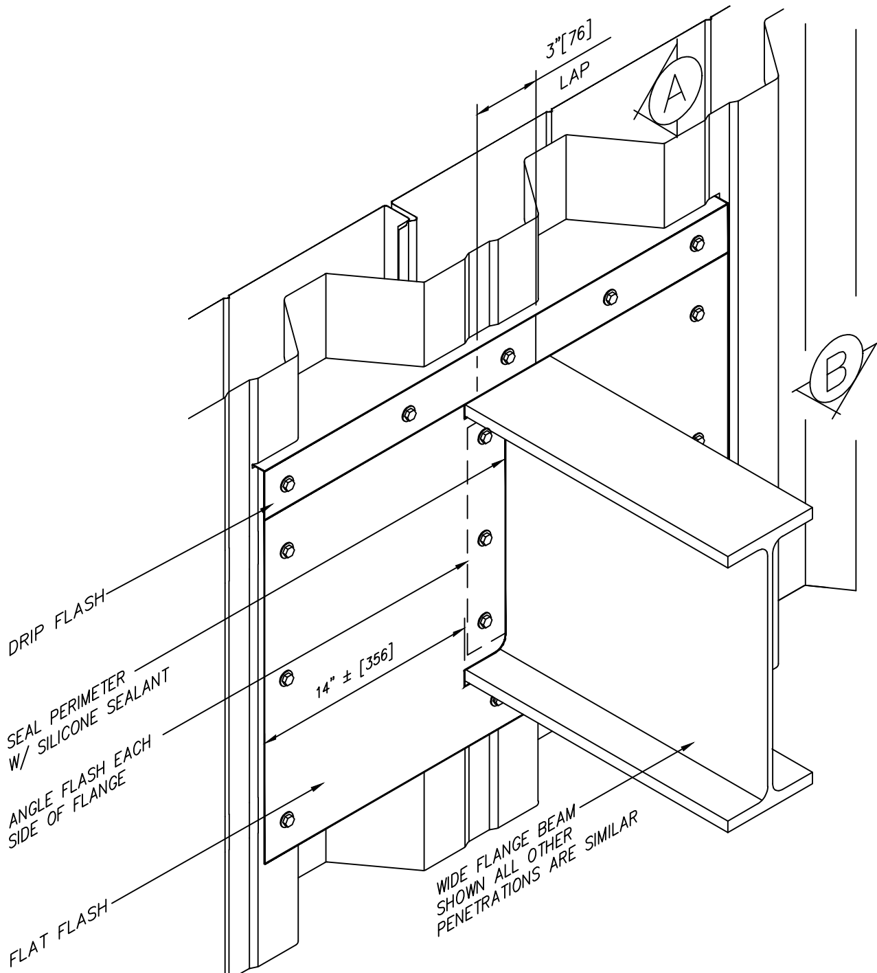
DETAIL 15 PENETRATION
