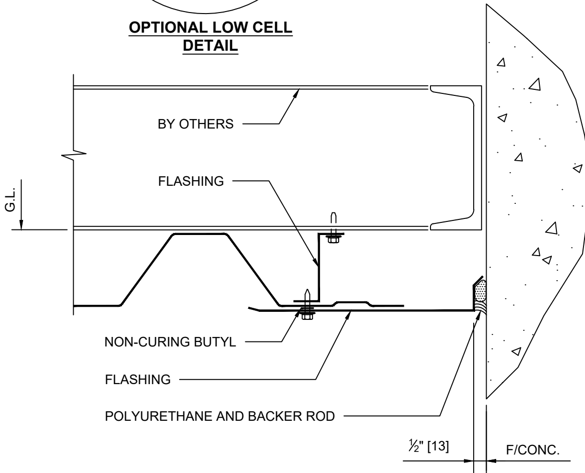
DETAIL 11 ENDWALL
