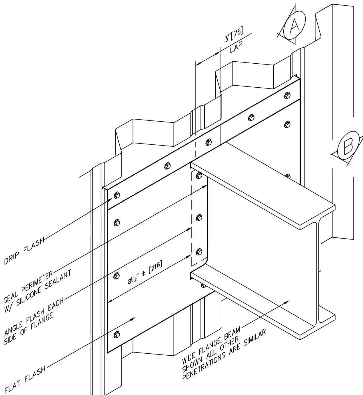
DETAIL 15 PENETRATION
