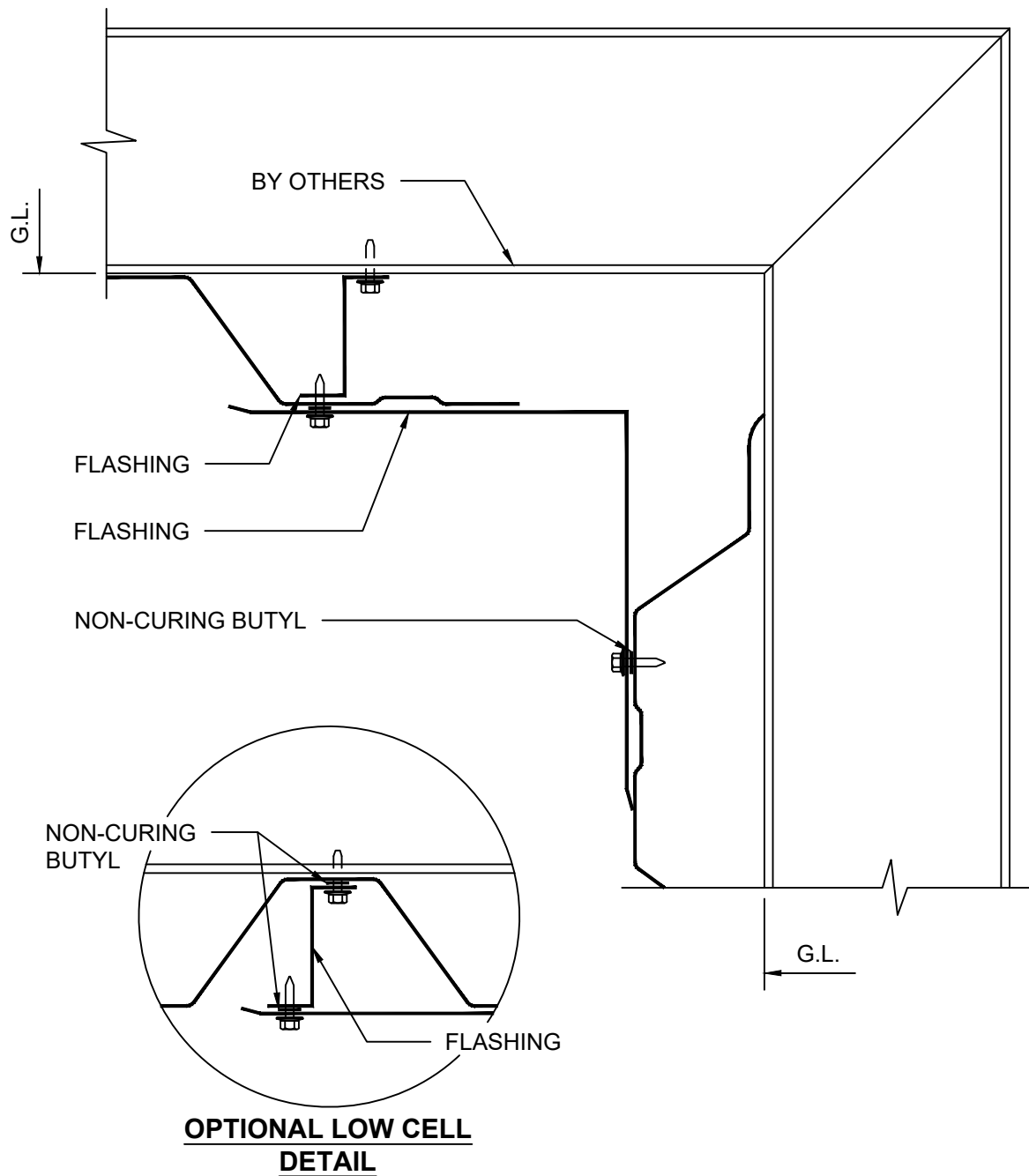
DETAIL 10 INSIDE CORNER
