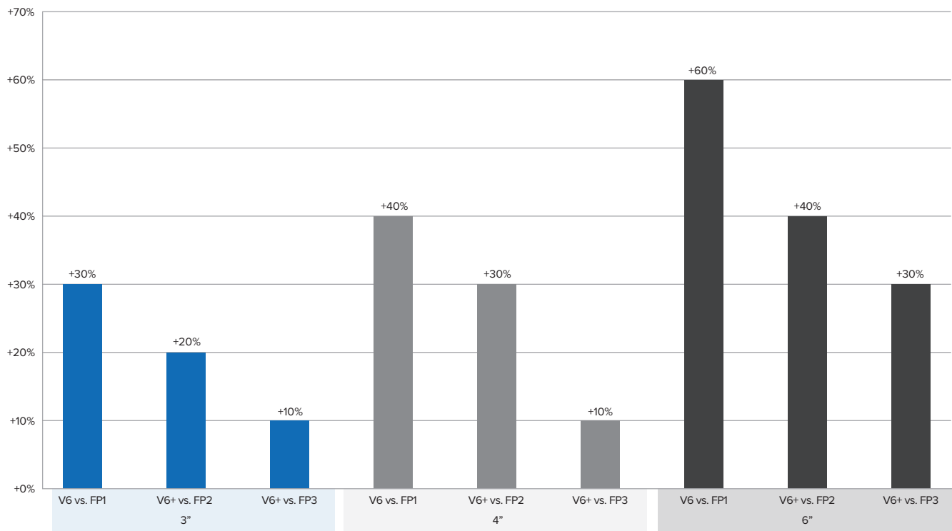
AVERAGE INCREASE IN ALLOWABLE SPAN: V6/V6+ vs. FP1/2/3
