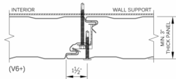
ONE V6 X-SPAN CLIP AT EACH SUPPORT WITH ONE FACE-TO-CLIP FASTENER AT EACH END SUPPORT
