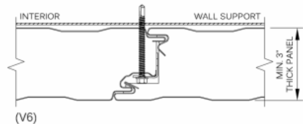
ONE V6 X-SPAN CLIP AT EACH SUPPORT
