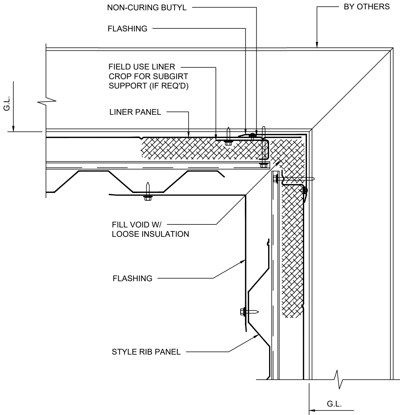
DETAIL 10 INSIDE CORNER - INSULATED
