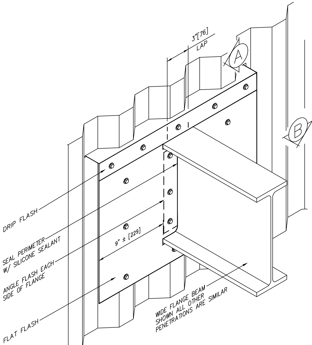
DETAIL 15 PENETRATION
