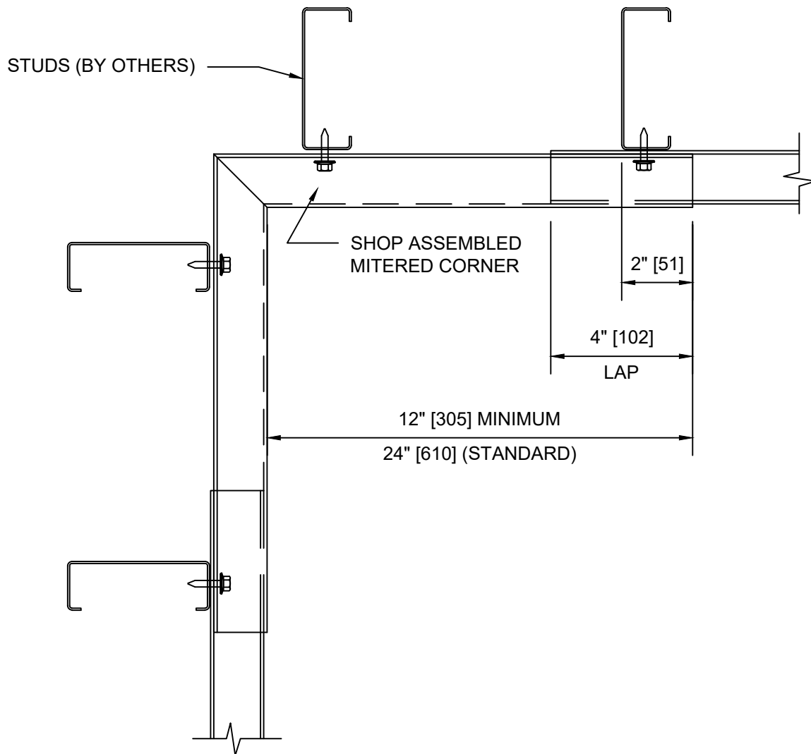
DETAIL 10A INSIDE MITERED CORNER
