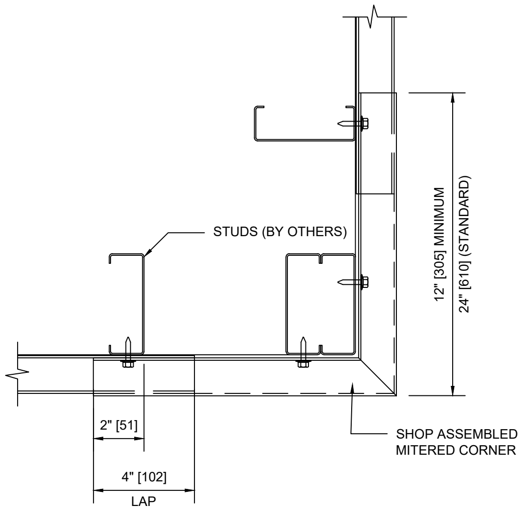
DETAIL 9A OUTSIDE MITERED CORNER
