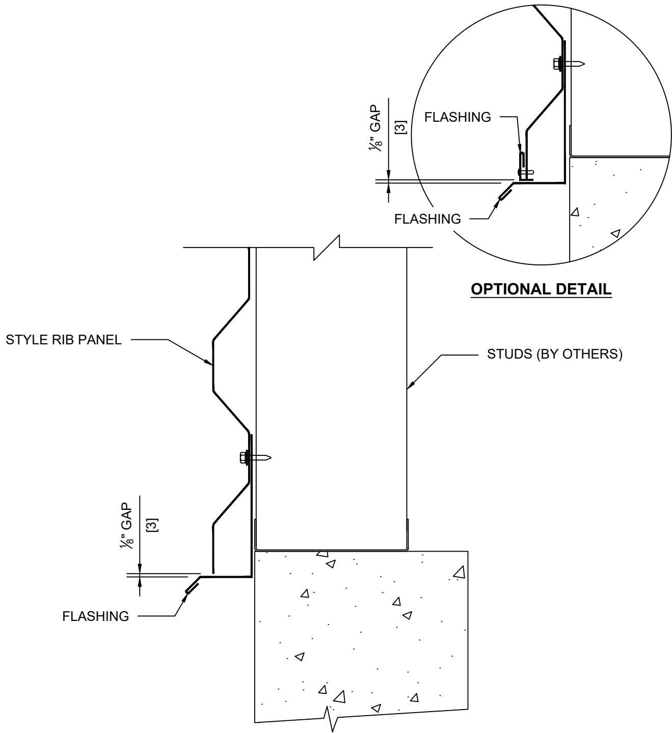
DETAIL 3B BASE AT CURB - HIGH CELL
