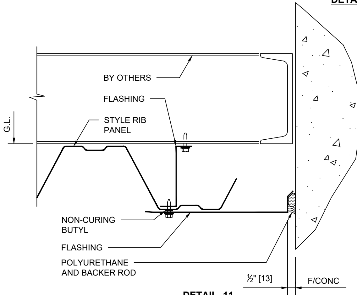
DETAIL 11 ENDWALL
