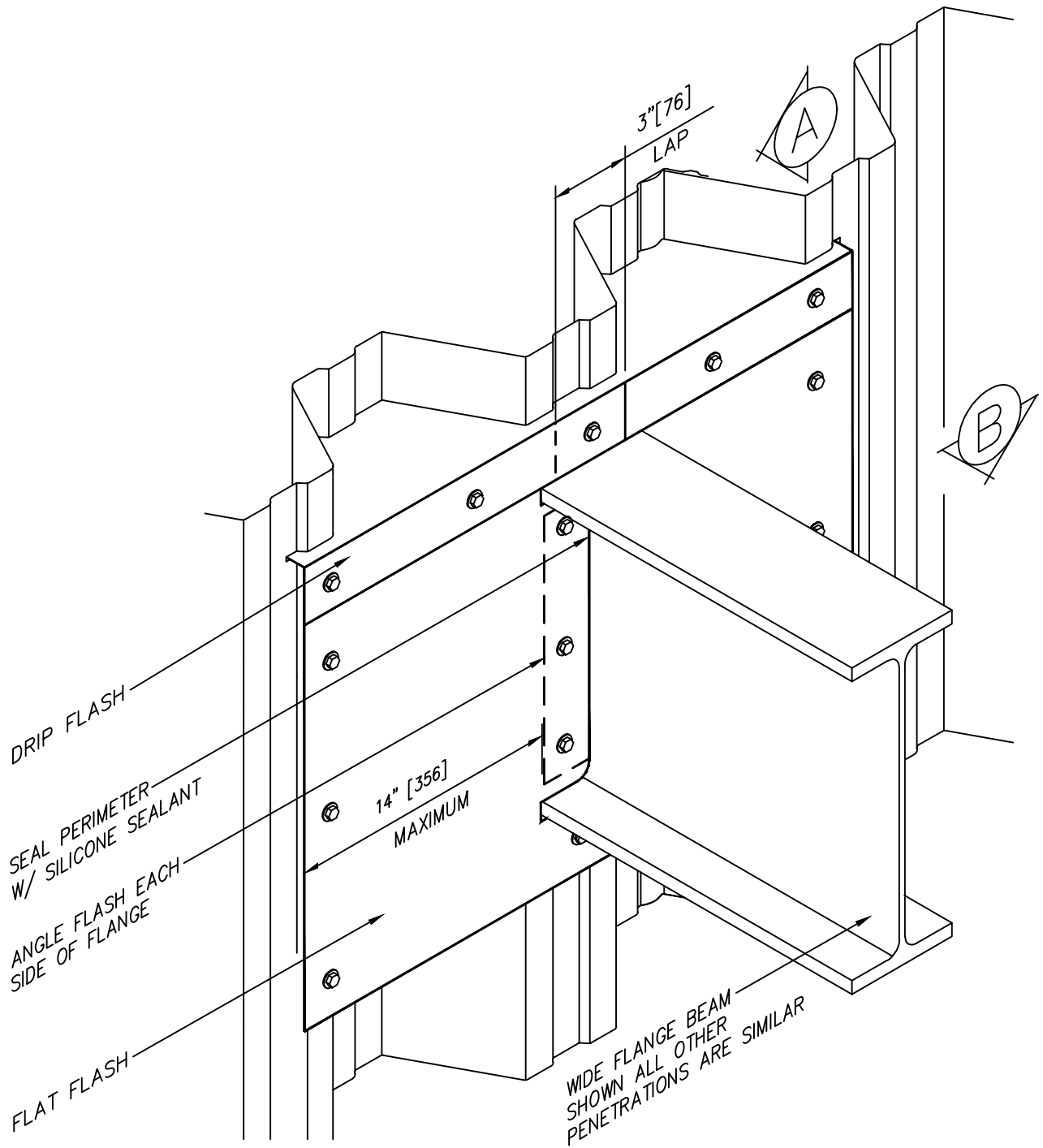
DETAIL 15 PENETRATION
