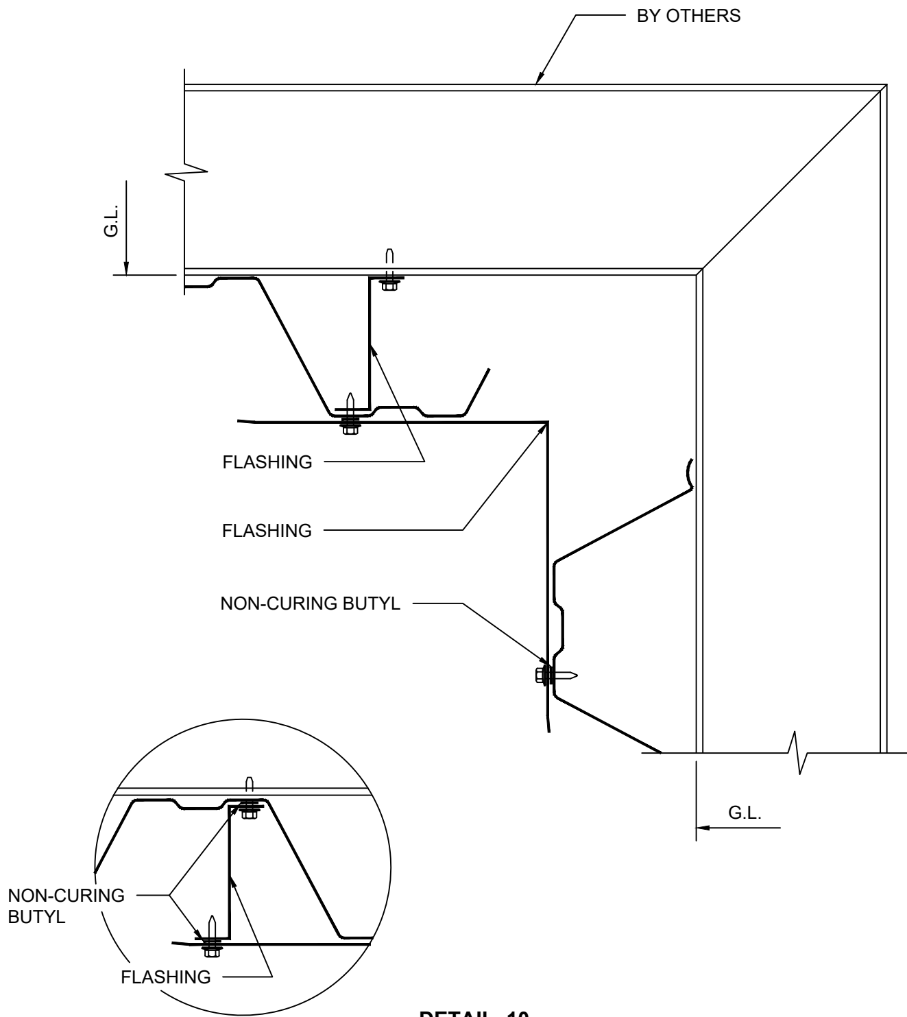
DETAIL 10 INSIDE CORNER
