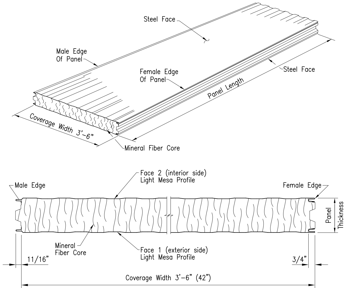
Panel Cross Section
