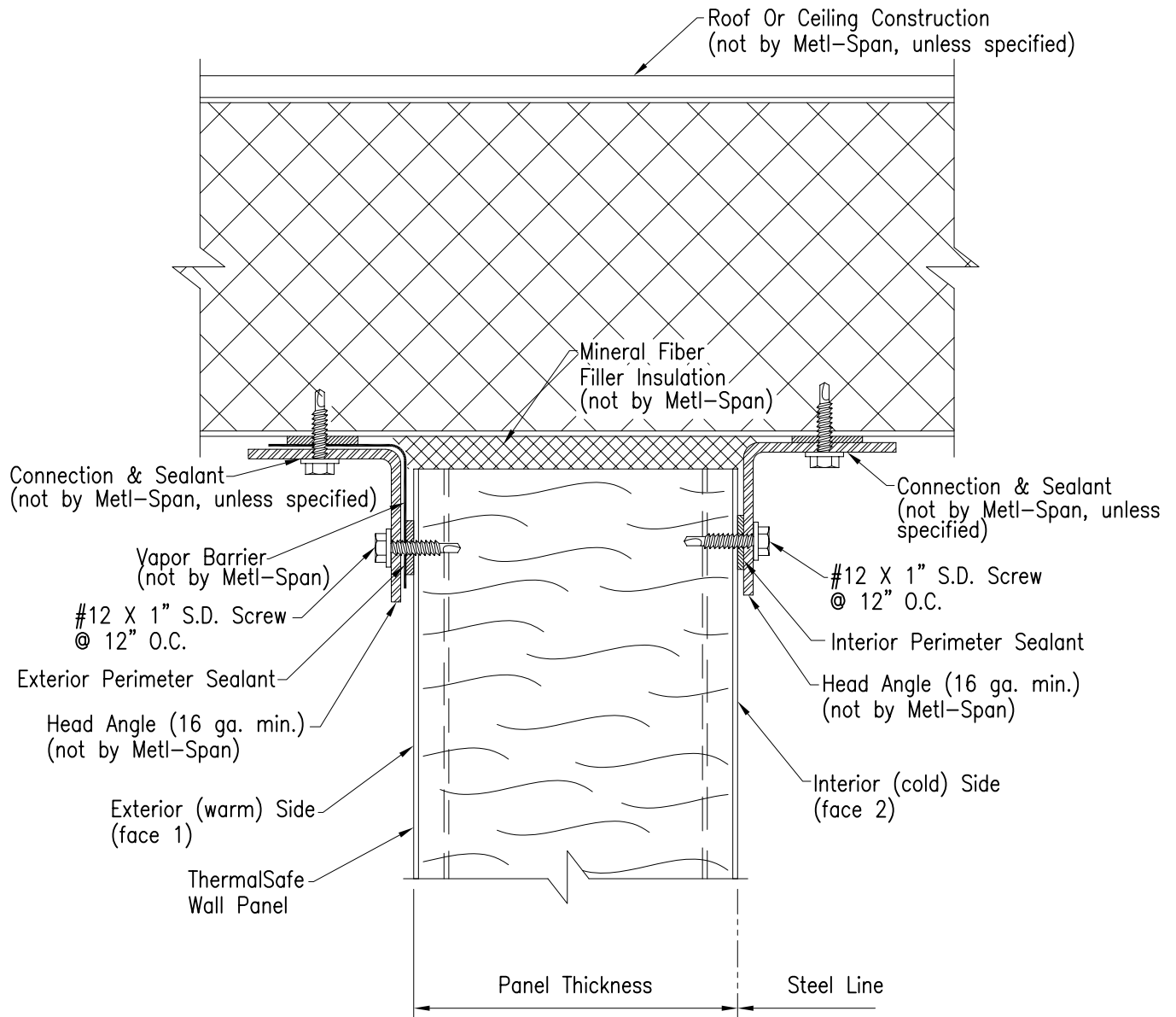
Vertical Panel-Head Detail (Isolated Head Angles)
