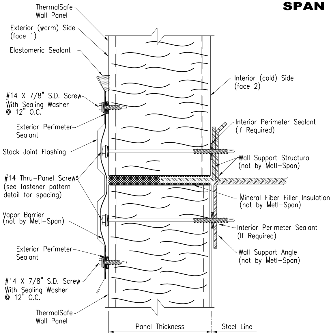
Vertical Panel-Stack Joint Detail
