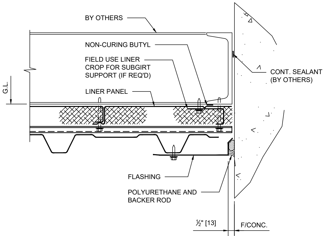
DETAIL 11 ENDWALL - INSULATED
