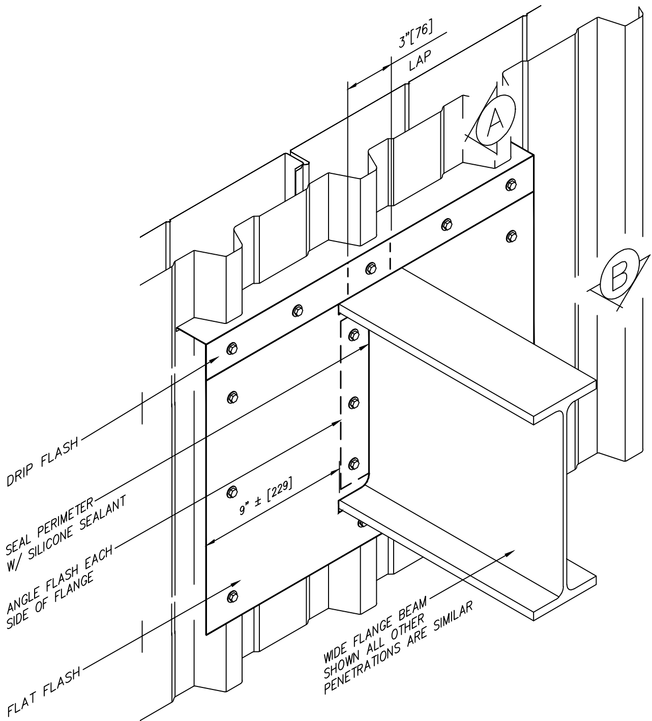
DETAIL 15 PENETRATION
