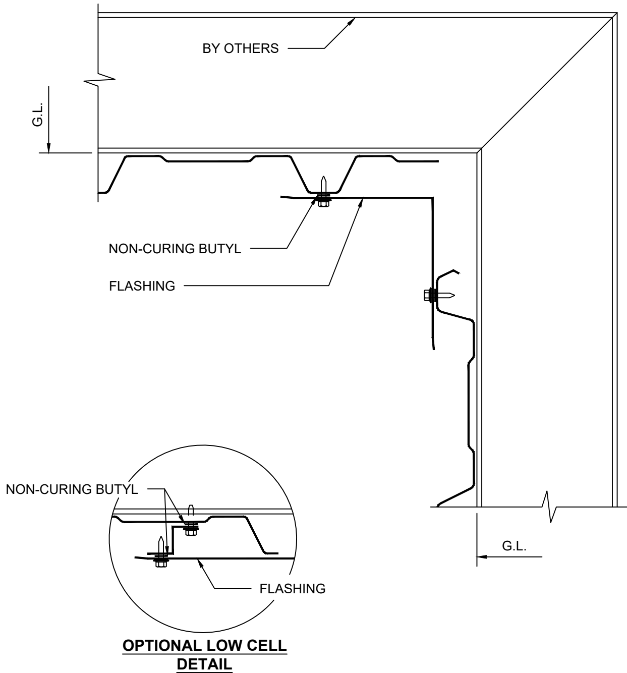
DETAIL 10 INSIDE CORNER
