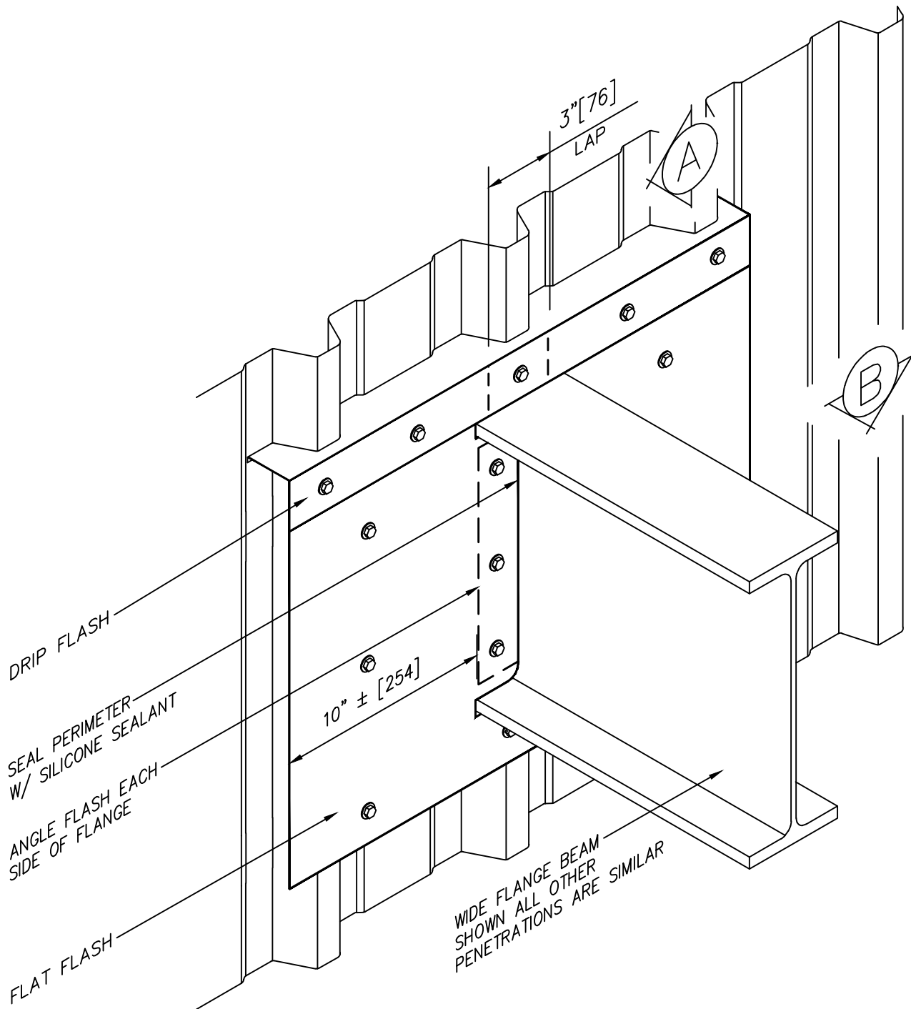
DETAIL 15 PENETRATION
